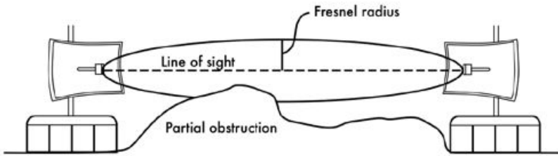
Figure RP 11: The Fresnel zone is partially blocked on this link, although the visual line of sight appears clear.
