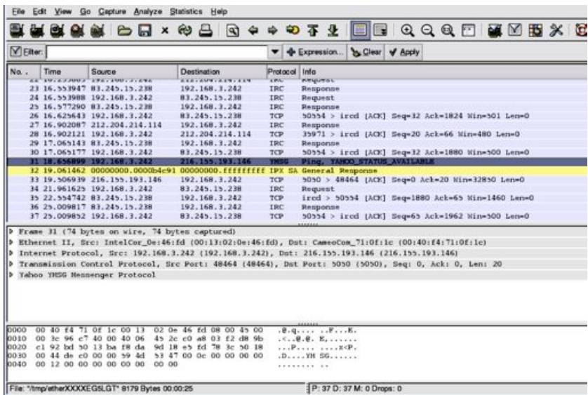
Figure NM 6: Wireshark (formerly Ethereal) is a powerful network protocol analyser that can show you as much detail as you like about any packet. Wireshark allows you to examine data from a live network or from a capture file on disk, and interactively browse and sort the captured data. Both summary and detailed information is available for each packet, including the full header and data portions.
