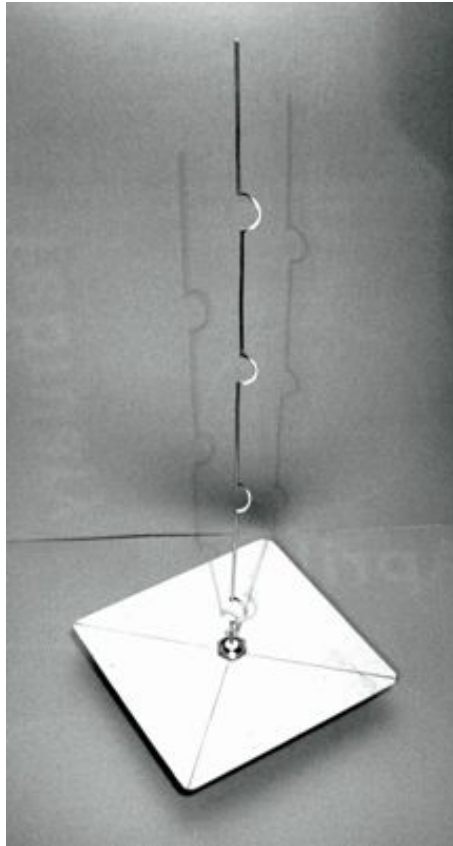
Figure AC 17: The finished antenna should be 42.5 cm from the plate to the end of the wire.
