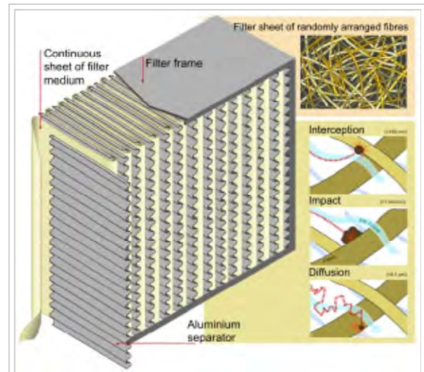
HEPA filter with functional description
