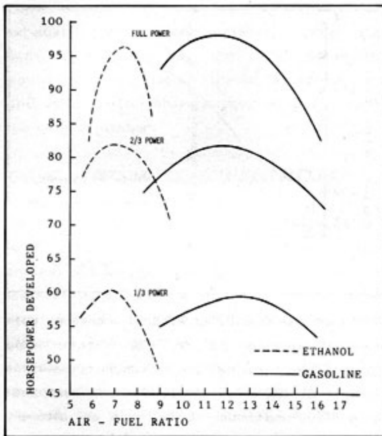
Figure 2-5 compares engine horsepower and air/fuel ratios for ethanol and gasoline in a six cylinder engine. The fuels in this case were 190 proof (95%) ethanol and "regular" gasoline having a specific gravity of 0.745. In the tests, air was supplied to the intake manifold at a constant 100 degrees Fahrenheit, and the carburetor needle valve was adjusted to provide the desired fuel/air ratios. The 2/3 and 1/3 loads were established by adjusting the throttle to give the same manifold pressure for both fuels.
