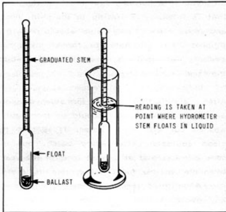
Figure 5-1: Hydrometer
