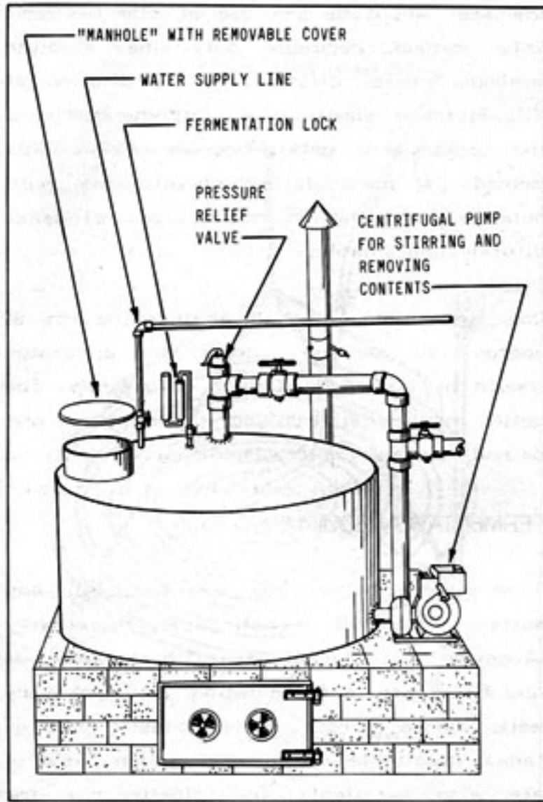
Figure 13-3: LARGE APPARATUS
