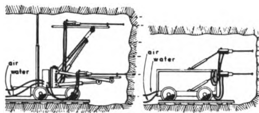
Figure 3.5. Jumbo
