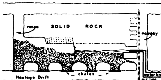
Figure 3.21. Shrinkage method
