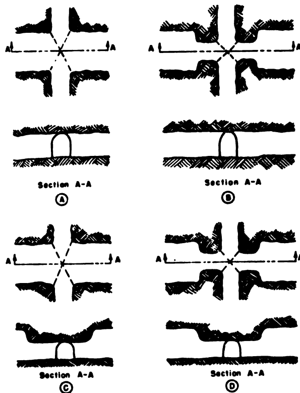
Figure 3.1. Tunnel intersections
