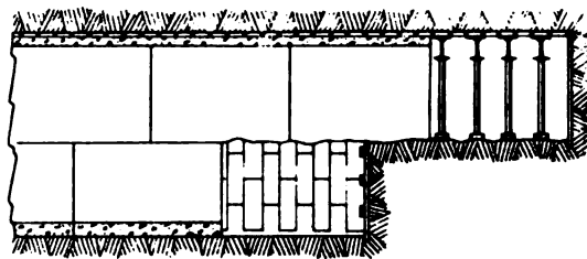
Figure 3.19. Flying arch method
