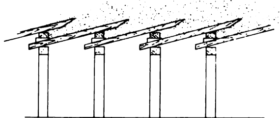
Figure 3.16. Method of forepoling
