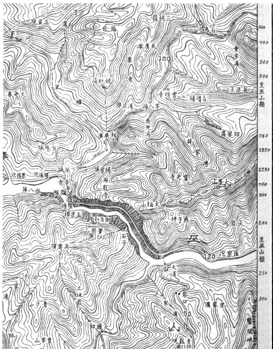
Figure 30. Section of Szechwan Province Map at 1:100,000 by the Chinese Survey Department, Combined Services Forces Headquarters, Ministry of National Defense. Figures in border are approximate contour-interval values in meters.
