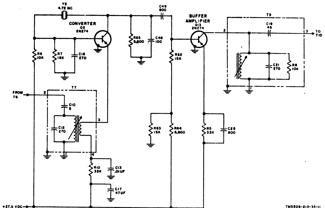
Figure 1. Converter and buffer amplifier, partial schematic diagram (R-1041A/ARN only).
