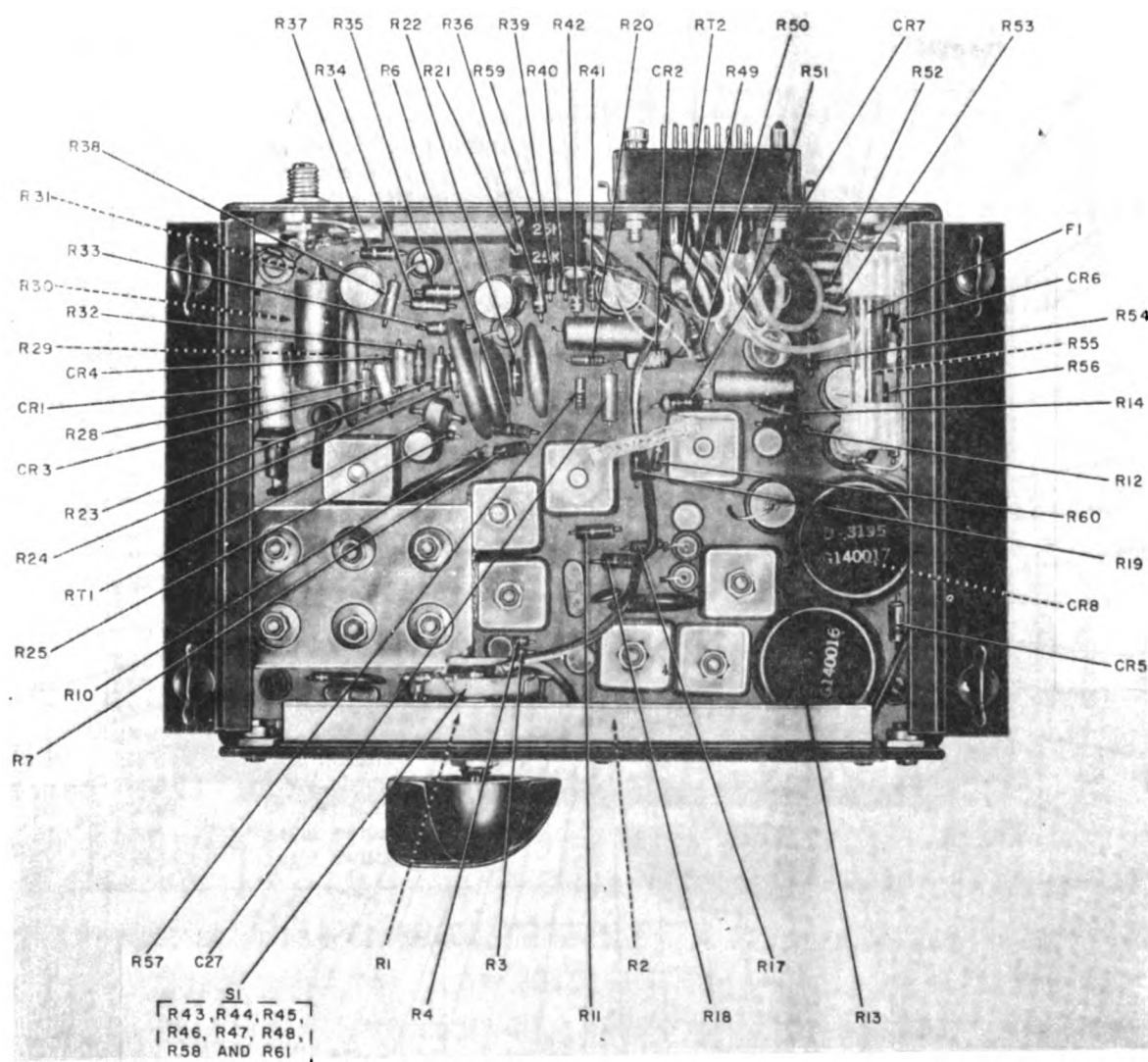
Figure 6. Receiver, Radio R-1041/ARN, top view, location of diodes and resistors.
