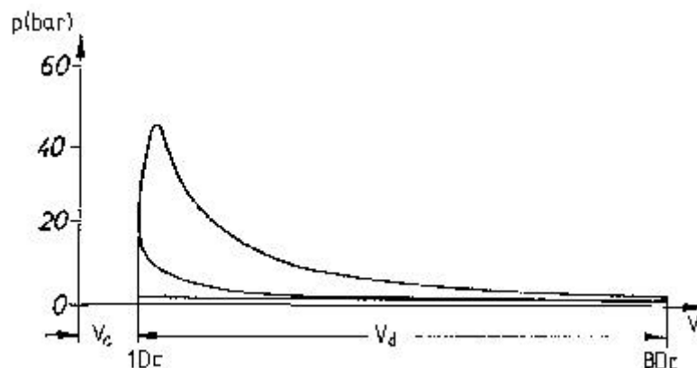
Fig. 3.14: Simplified p, v-diagram of an Otto process
