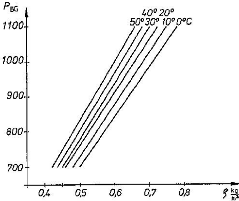
Fig. 4.1: Density r of \text{CH}_4 as a function of biogas pressure and temperature
