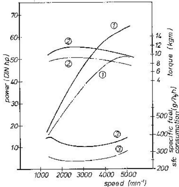
Fig. 6.1: Performance diagram of an Otto engine using liquid fuel (—) and methane(---) alternatively (Rodagas).
