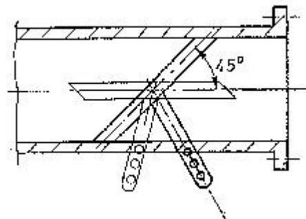
Fig.5.10: Butterfly gas control valve with elliptic butterfly for small angular movement ( 45^\circ )
