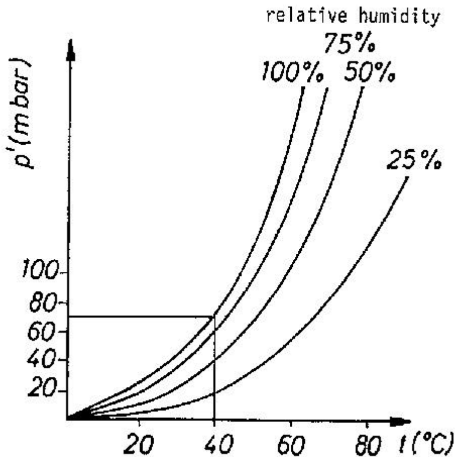
Fig. 4.3: Partial pressure of water vapor in a mixture with biogas as a function of a biogas temperature and relative humidity
