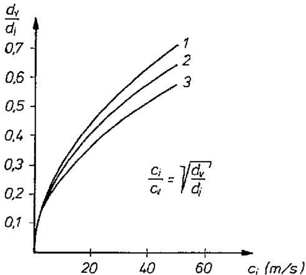
Fig. 6.5: Venturi diameter ratio d_v/d_i as a function of intake velocity c_i and the required velocity at the venturi bottleneck c_v
