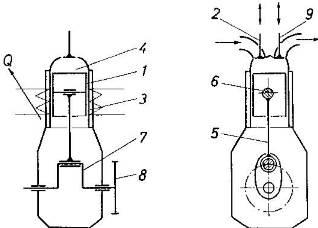
Fig.31:Principal scheme of a 4-stroke engine.1 piston, 2 inlet valve, 3 cylinder, 4 combustion chamber, 5 connection rod, 6 gudgeon pin, 7 crankshaft, 8 flywheel, Q head rejected (cooling).
