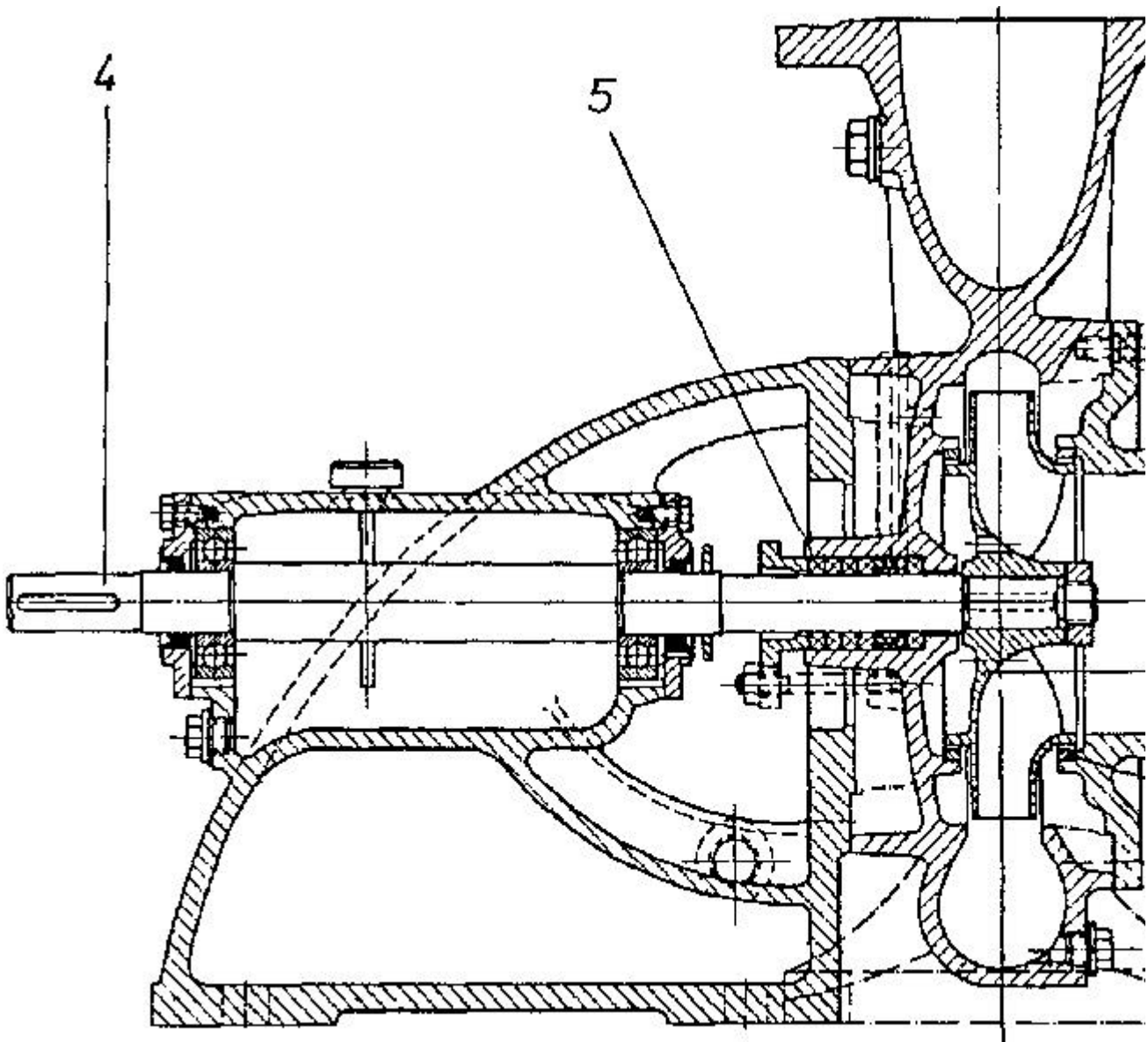
Fig. 7.11: Cross-sectional view of single-stage centrifugal pump (KSB).
