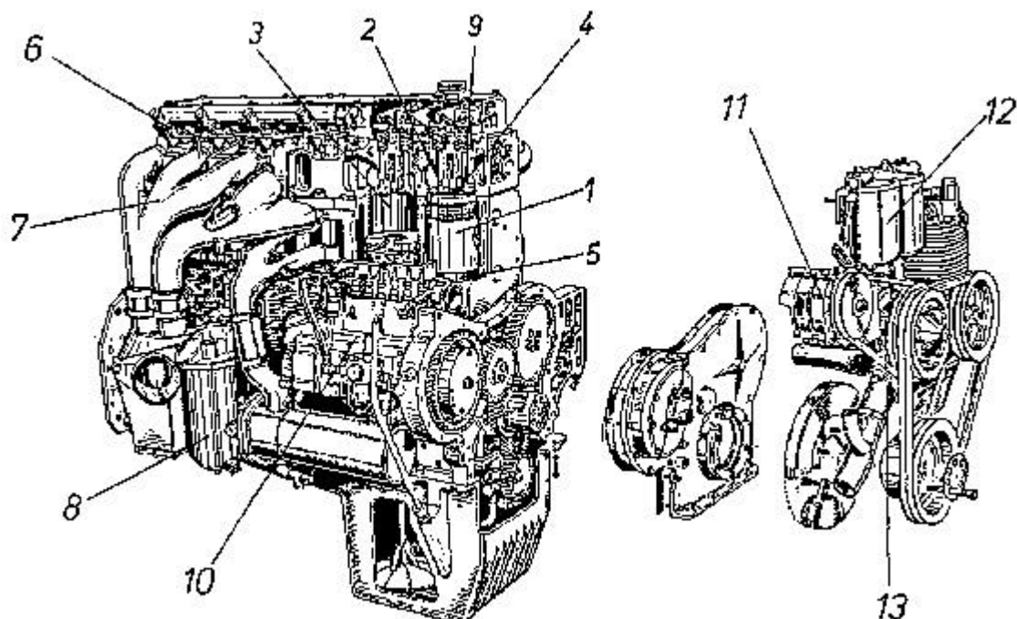
Fig. 3.7: 6-cylinder diesel engine, partly opened (MAN).
