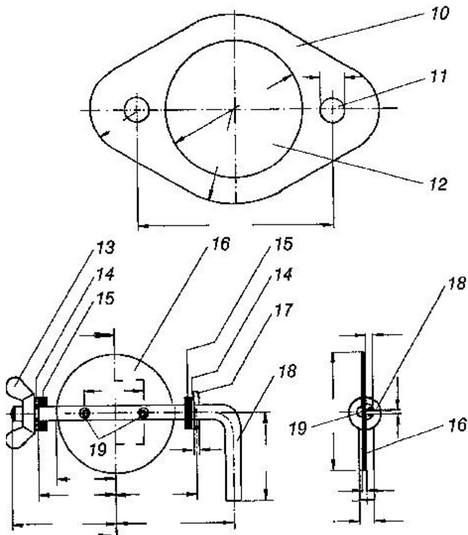
Fig. 2: Venturi mixer parts, continued. 10 Connection flange, 11 Bore for connection bolts to engine and air filter, 12 Bore for connection of mixer body (brazed, welded), 13 Wing nut for fixing the butterfly valve shaft, 14 Washer, 15 Rubber/plastic seal ring, 16 Butterfly valve, 17 Washer fixed to butterfly valve shaft, 18 Butterfly valve shaft cum control lever, 19 Small bolts for fixing butterfly to shaft.
