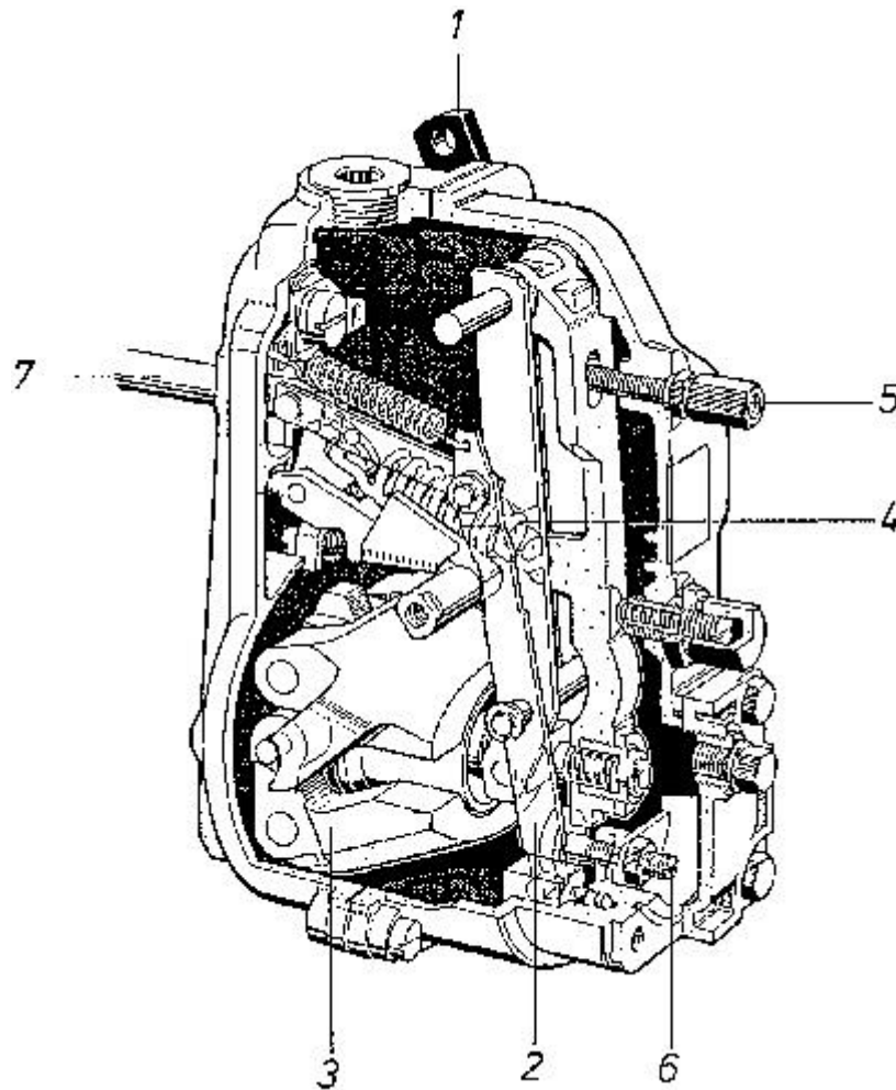
Fig. 5.8: Governor for diesel fuel injector pump (Bosch).
