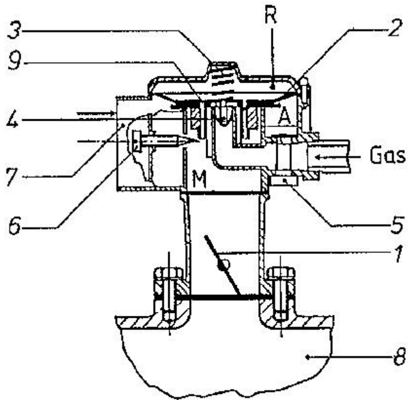
Fig. 6.6: Cross-sectional view of gas mixing valve.
