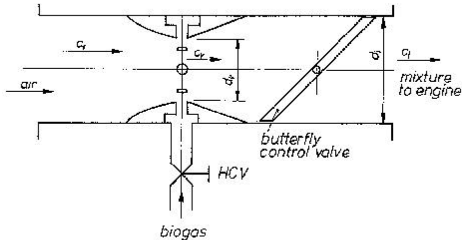
Fig. 6.2: Venturi mixer with gas supply through several bores.
