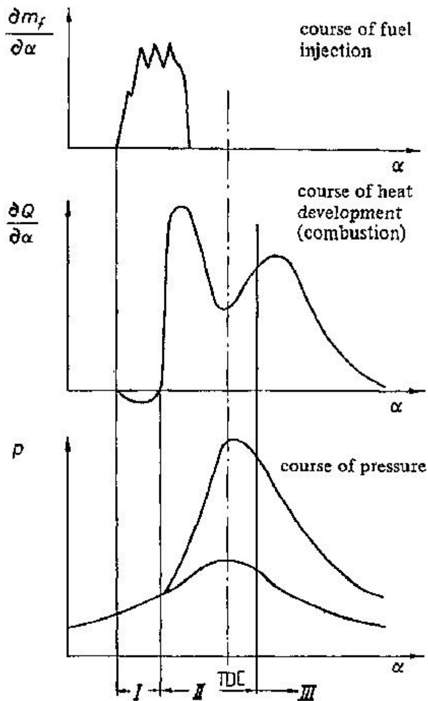
Fig. 3.9: Courses of fuel injection, combustion and pressure as a function of the crank angle \alpha
