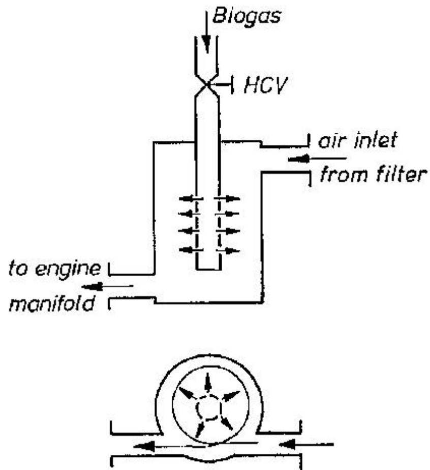
Fig.5.2: Simple mixing chamber with hand - controlled valve (HCV)
