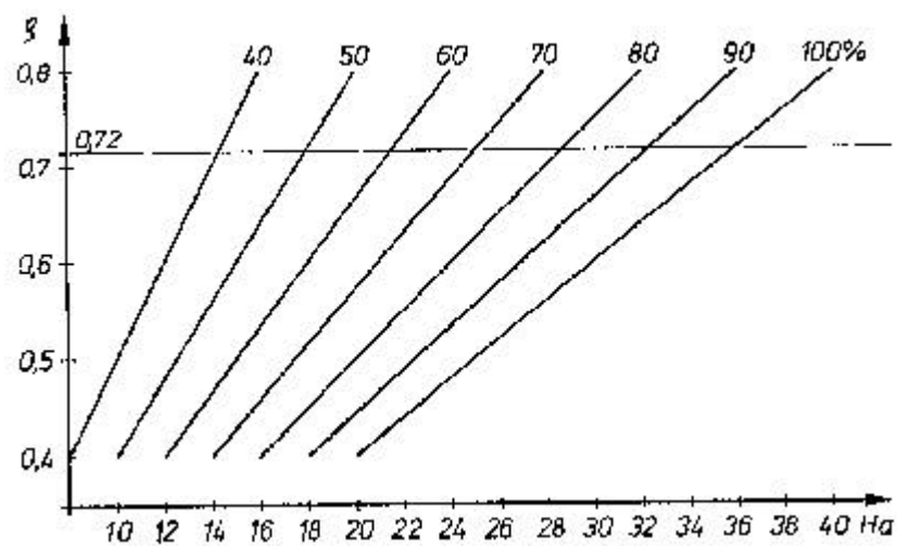
Fig. 4.2: Calorific value of biogas as a function of the density and volume %-age of its \text{CH}_4 content ( r = 0.72 is the density at a standard condition)
