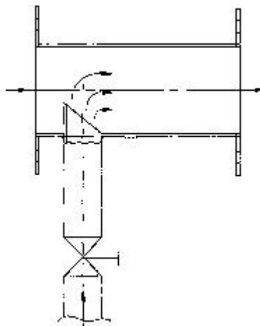
Fig. 5.4: T-joint mixer with oblique, protruding gas inlet
