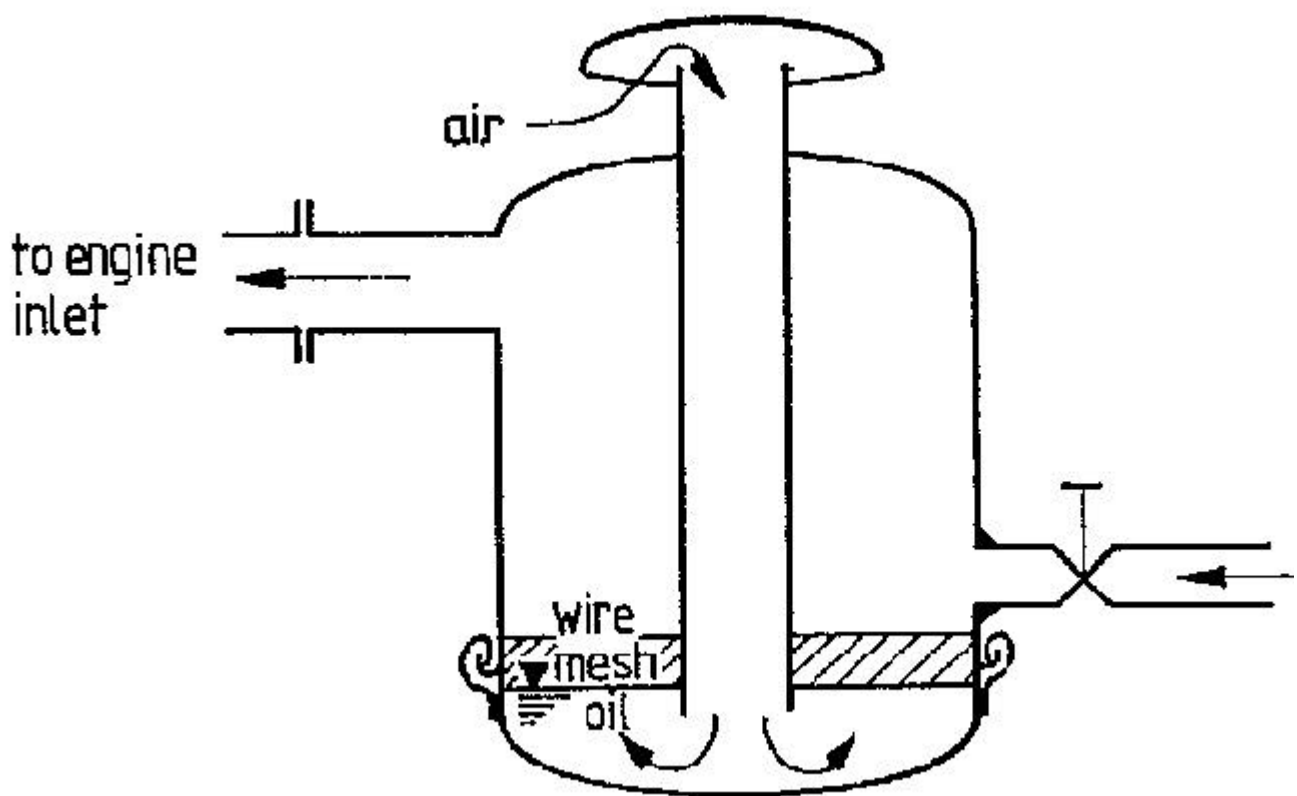
Fig. 5.3: Air filter modified into mixing chamber
