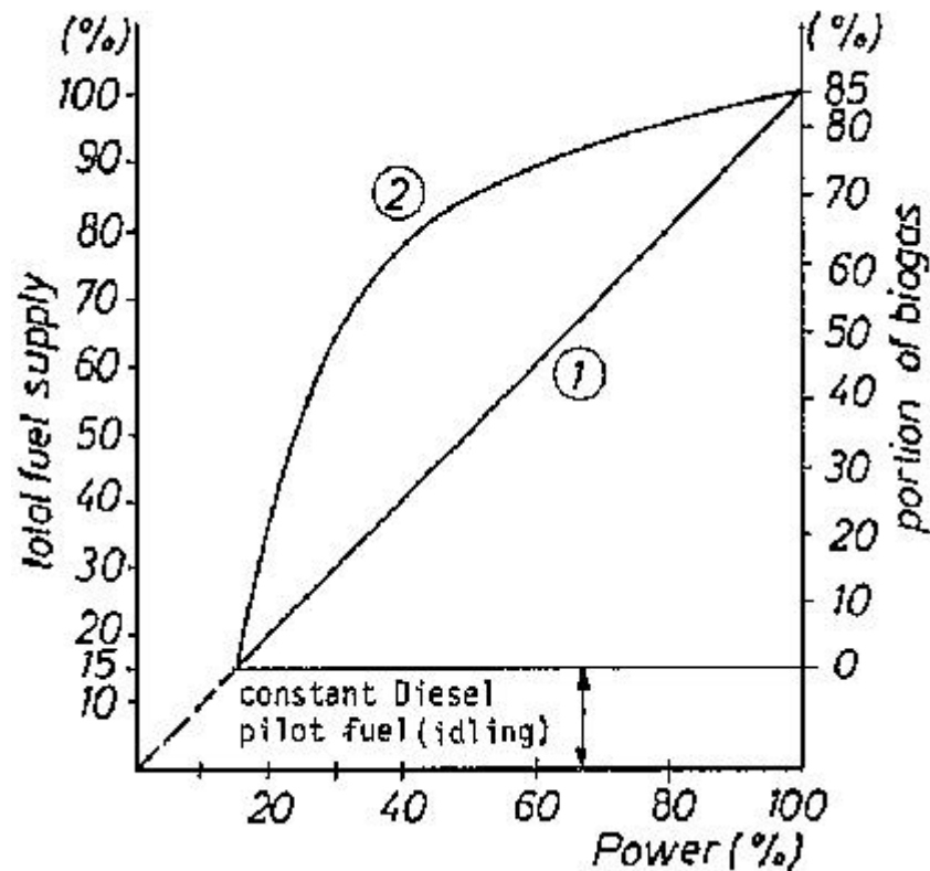
Fig. 5.9: Fuel supply vs. power output Diesel pilot fuel constant, biogas controlled (manually or automatically) according to power demand.
