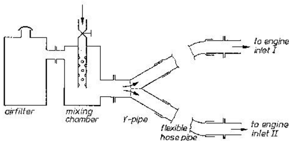
Fig.5.7: Mixing chamber connected to a V-type engine (engine)
