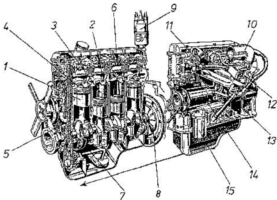
Fig. 3.13: Otto engine, partly opened (BMW).
