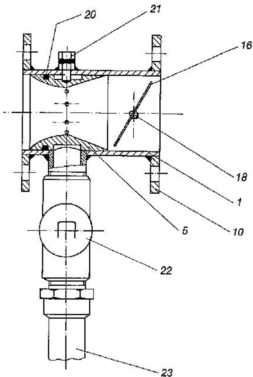
Fig. 3: Venturi mixer assembly
