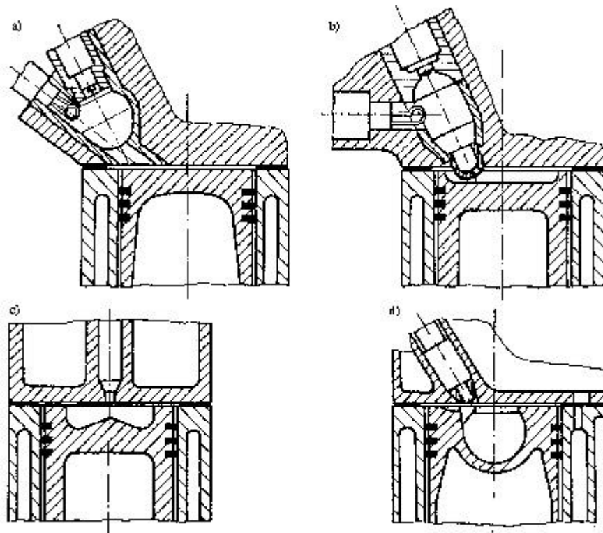
Fig. 3.12: Different combustion chamber forms and methods of fuel injection.
