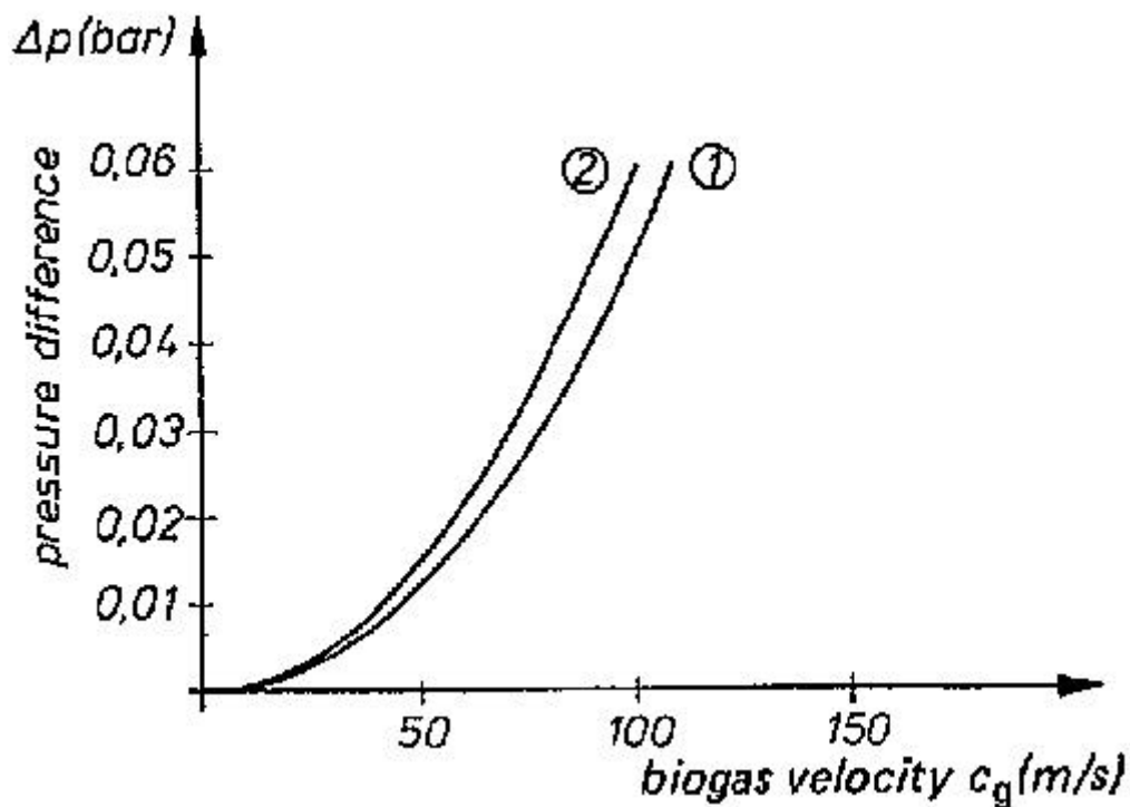
Fig. 6.4: Biogas flow through a nozzle c_g as a function of the active pressure difference \Delta p .
