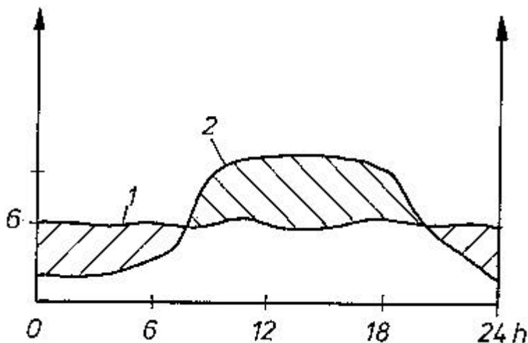
Fig 24: Daily profiles: 1 biogas and potential power production, 2 power demand; option for storage of excess biogas for periods of biogas shortage. /// excess biogas production \biogas shortage
