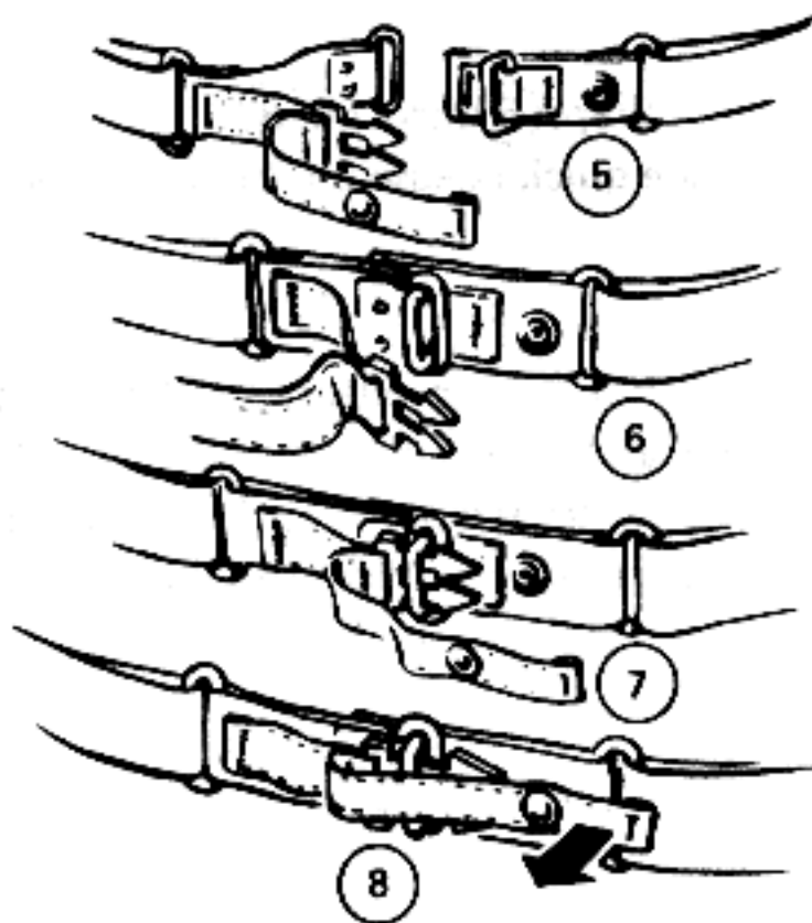
WAIST STRAP QUICK RELEASES
