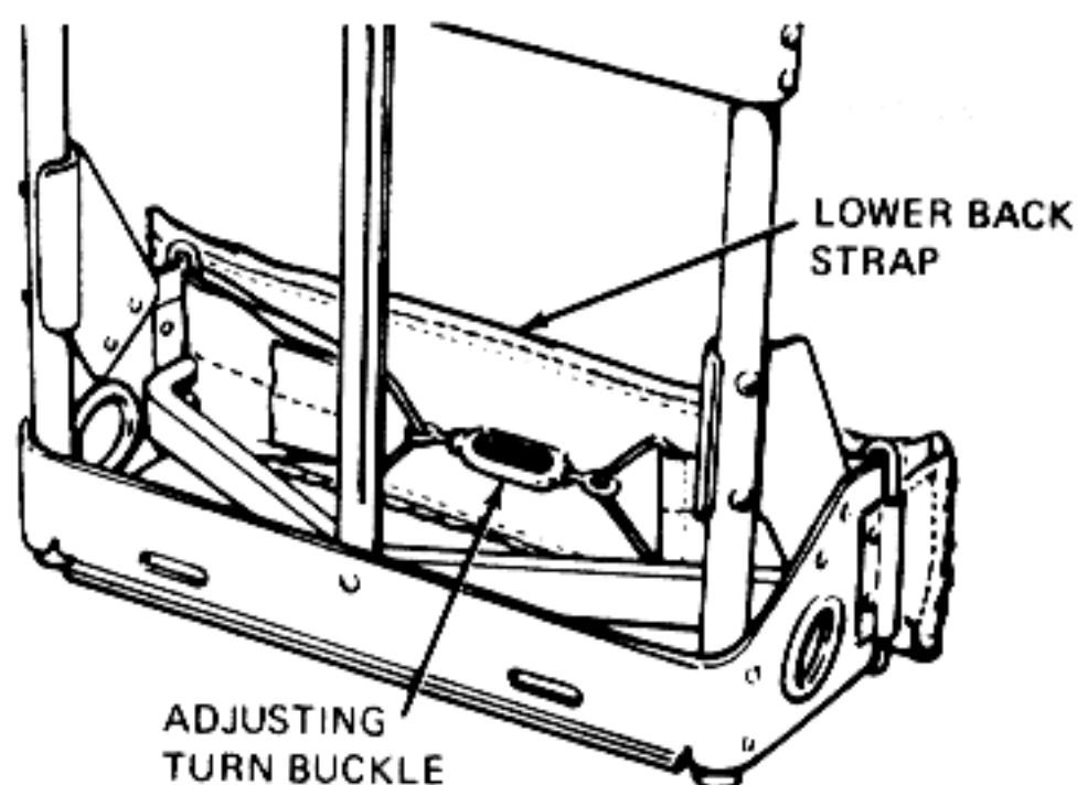
Figure 9. Lower Part of Pack Frame
