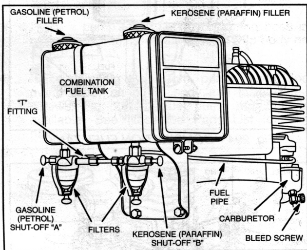
Fig. 298 – COMBINATION FUEL TANK
