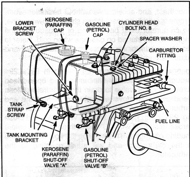
Fig. 297 – COMBINATION FUEL TANK
