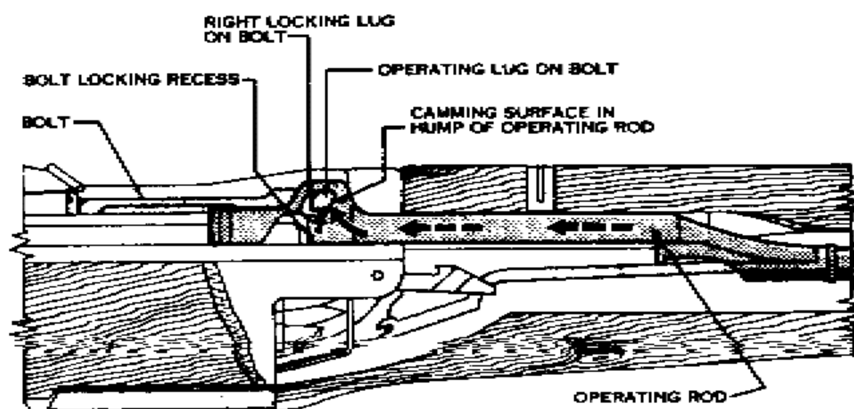
Fig. 53. Unlocking.
