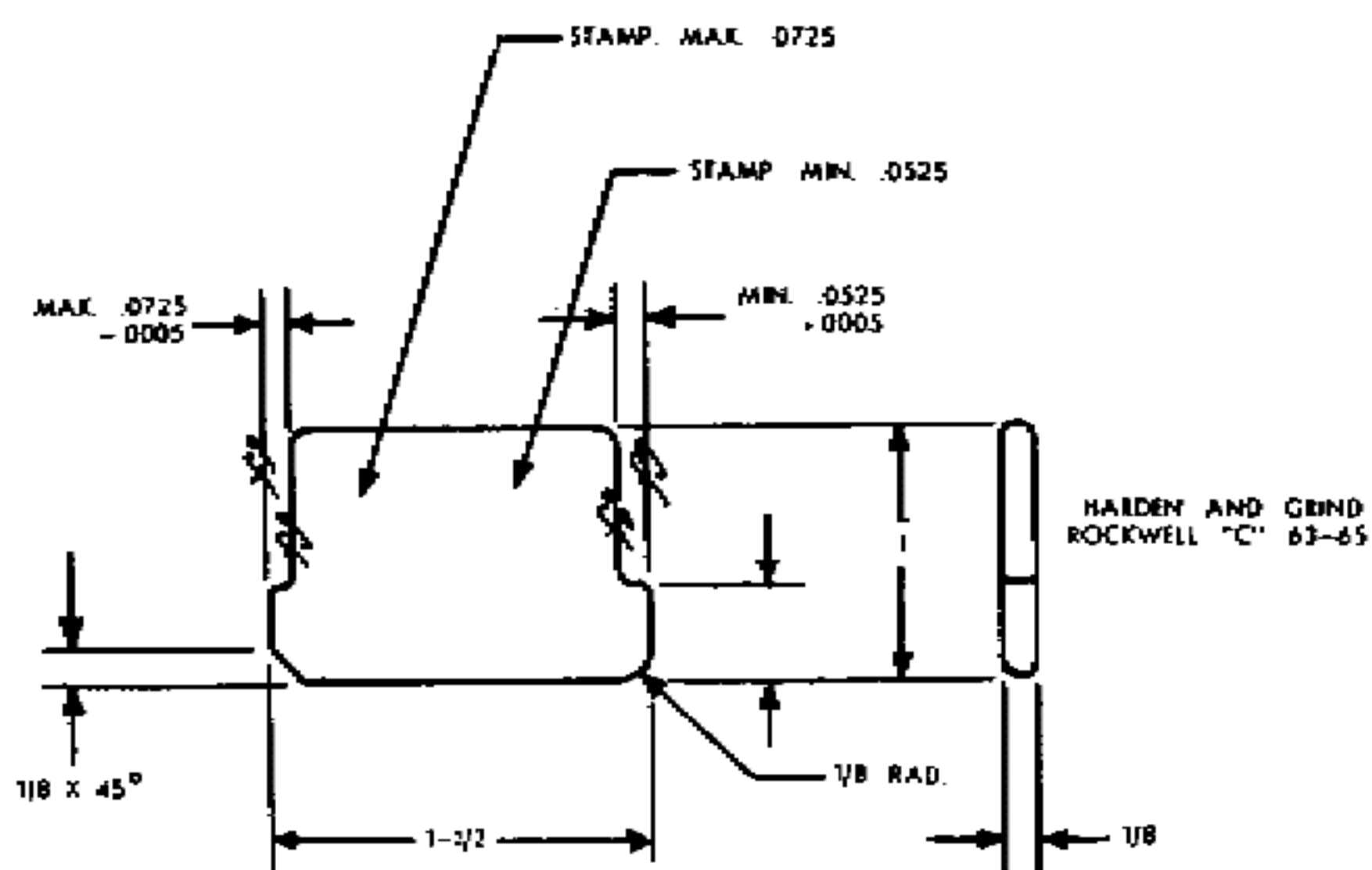
Fig. 109. Height gage.
