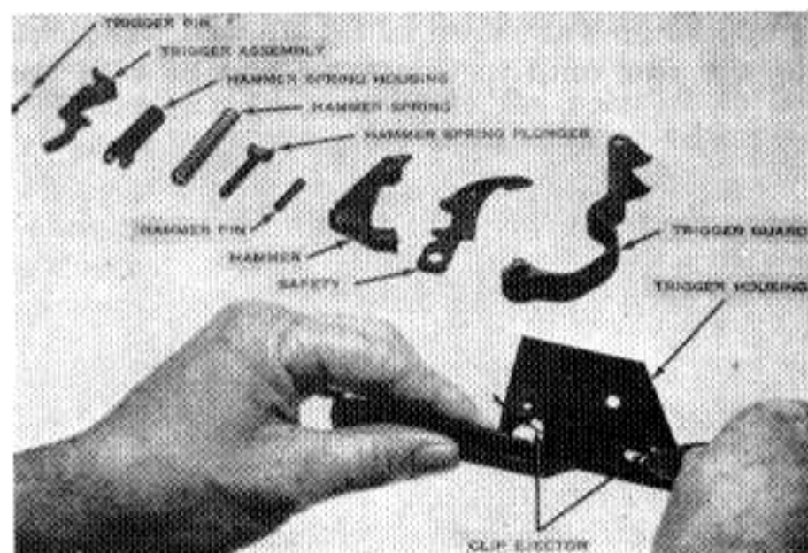
Fig. 77. Removing the clip ejector, other parts shown in order of disassembly.
