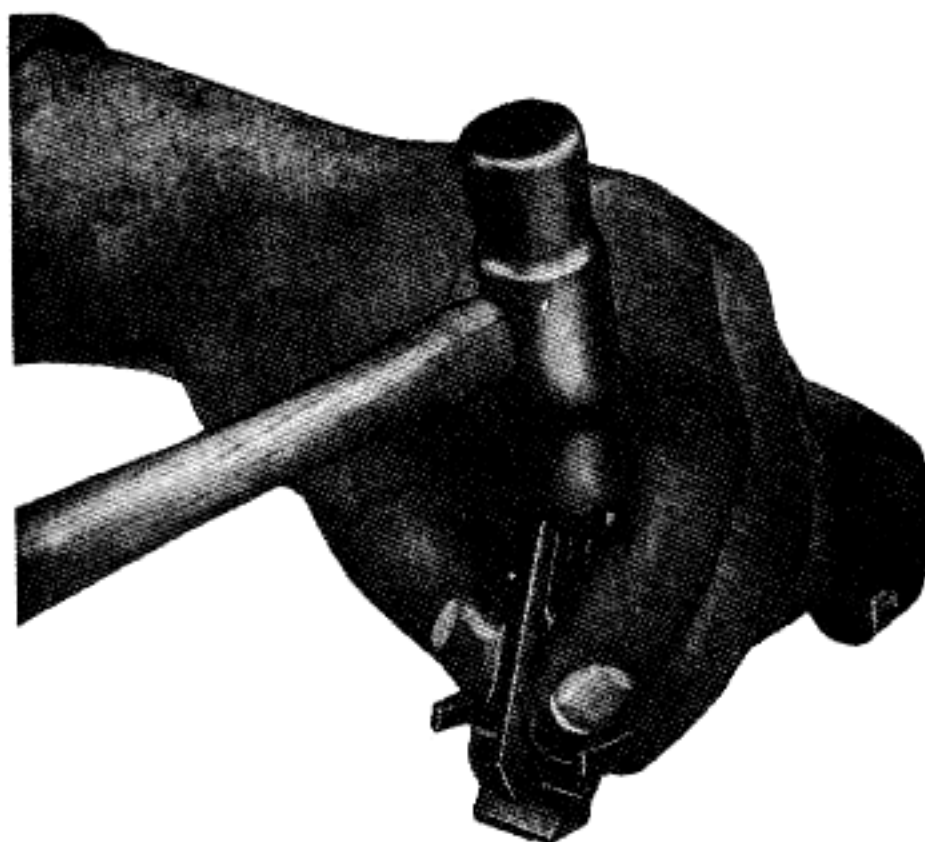
Fig. 143. Assembling follower.
