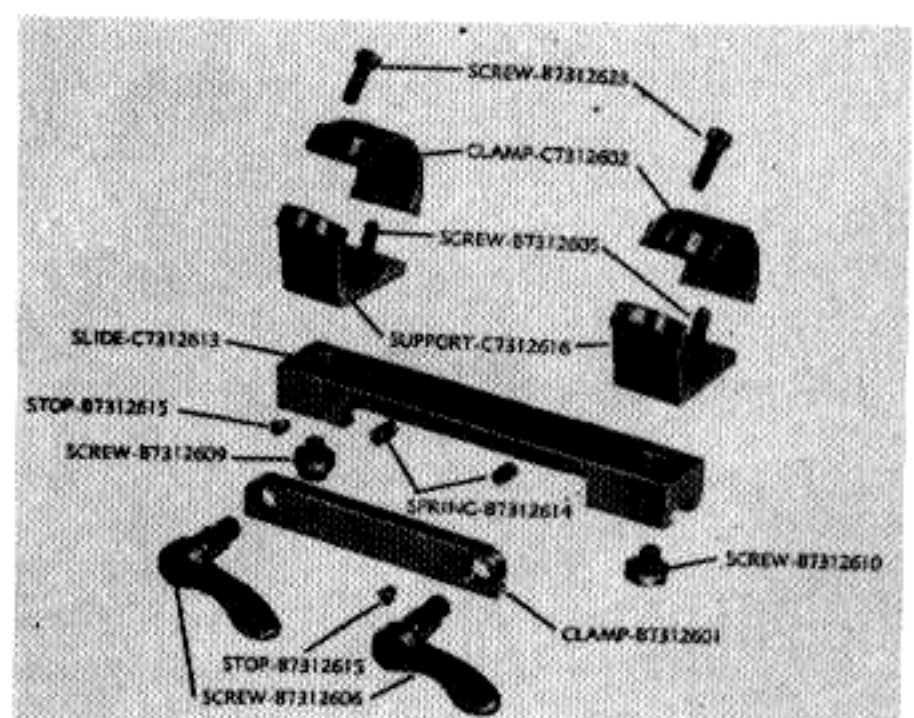
Fig. 129. Scope mount assembly, M1C.
