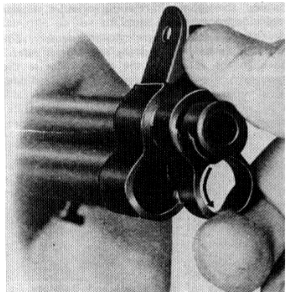
Fig. 82. Removing the gas cylinder lock.
