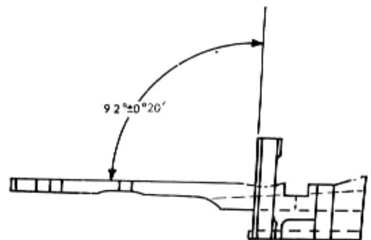
Fig. 123. Follower showing correct angle.
