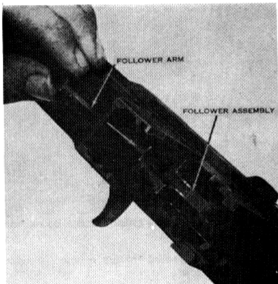
Fig. 86. Replacing the follower arm.
