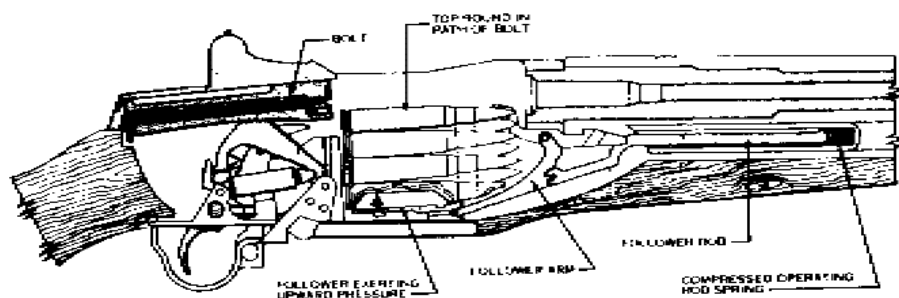
Fig. 48. Position of parts, bolt in rearmost position.
