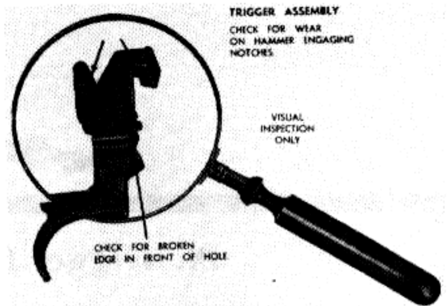
Fig. 149. Points to inspect on trigger assembly.
