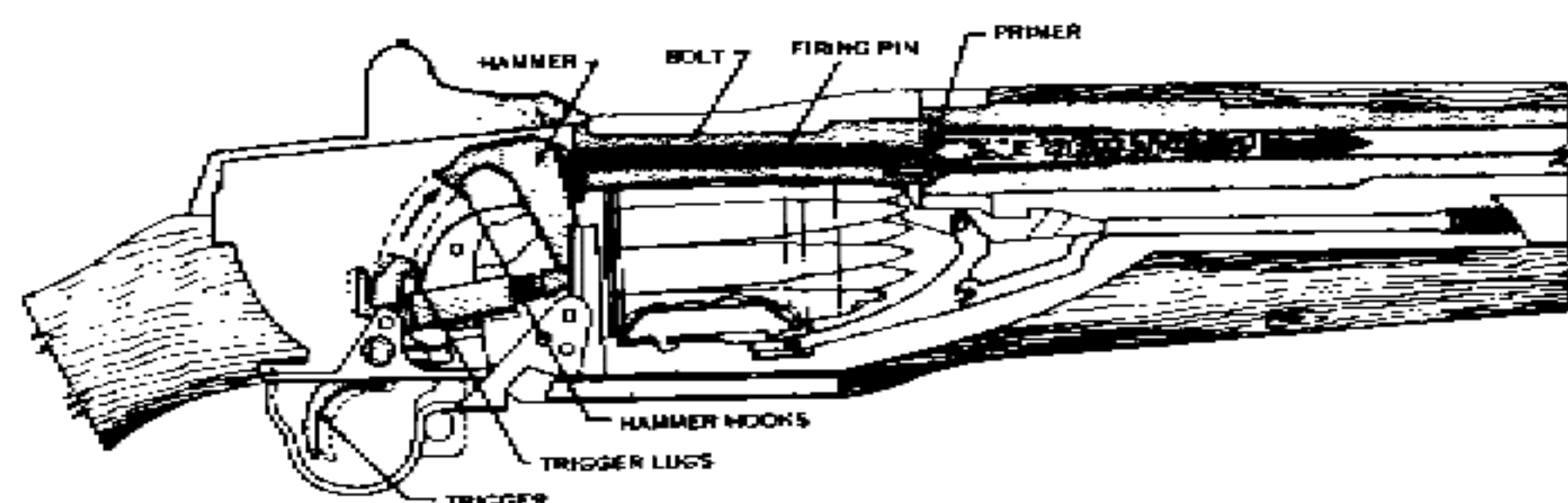
Fig. 51. Firing.
