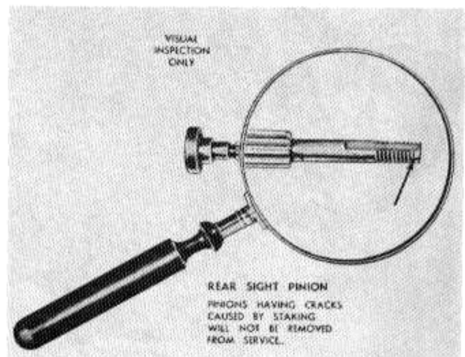
Fig. 124. Rear sight pinion - early manufacture.
