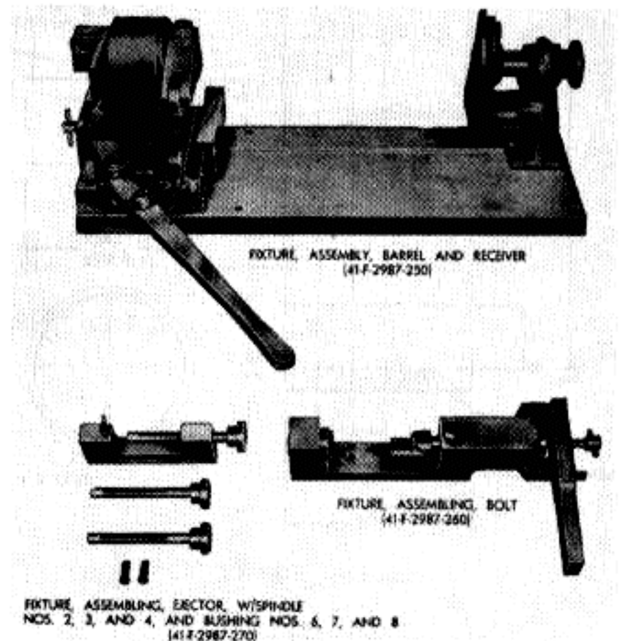
Fig. 103. Fixtures.
