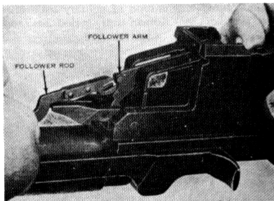
Fig. 87. Replacing the follower rod and operating rod spring.
