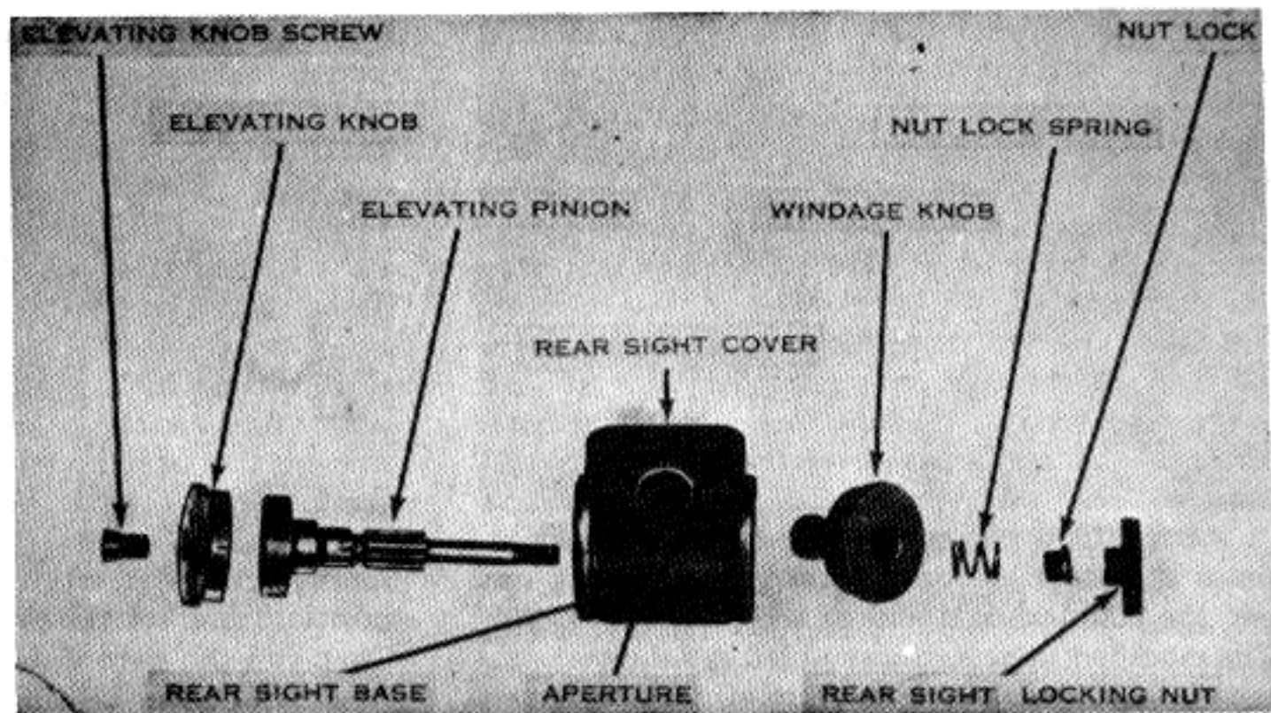
Fig. 69. Parts of old rear sight.
