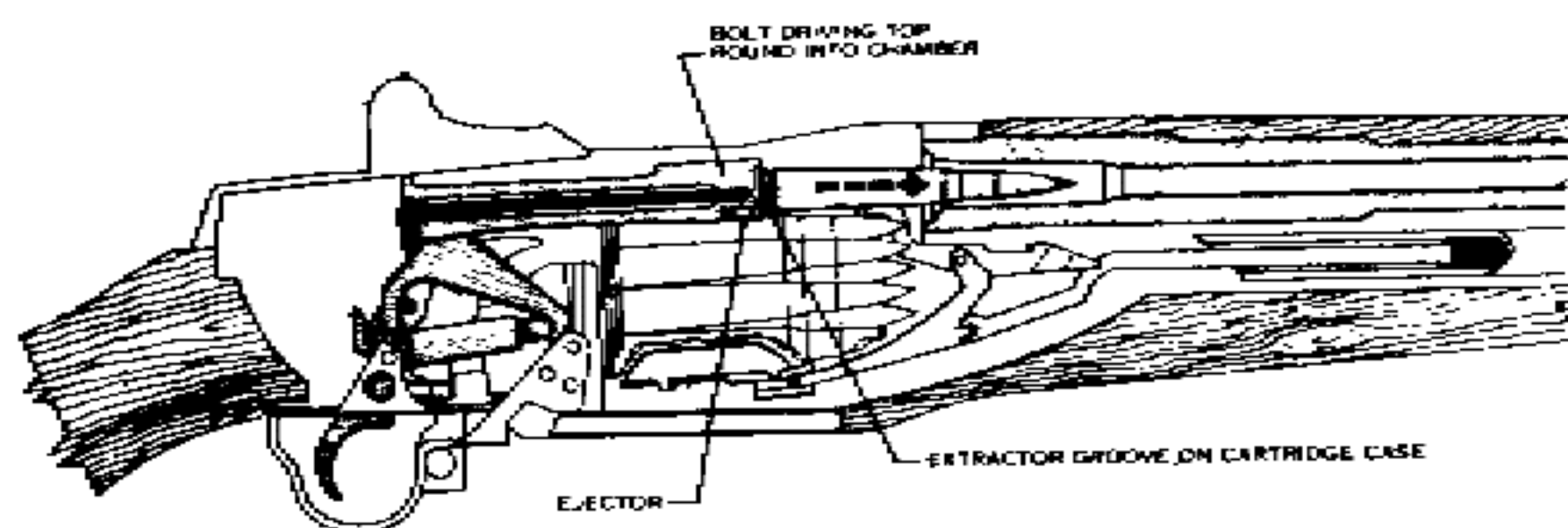
Fig. 49. Chambering.
