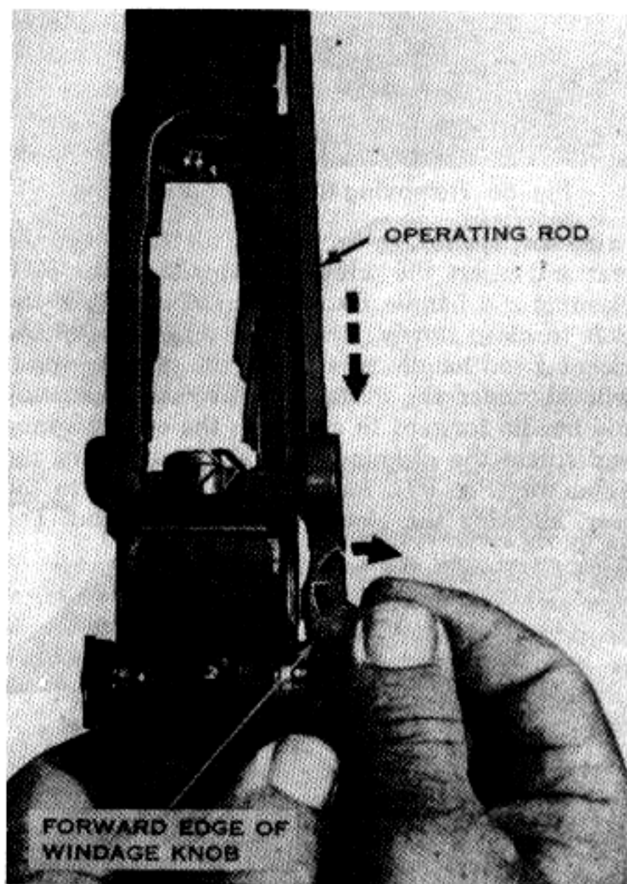
Fig. 64. Removing the operating rod.
