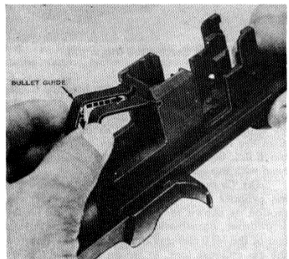
Fig. 84. Replacing the bullet guide.
