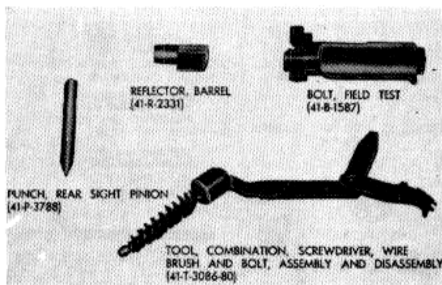
Fig. 100. Tools.
