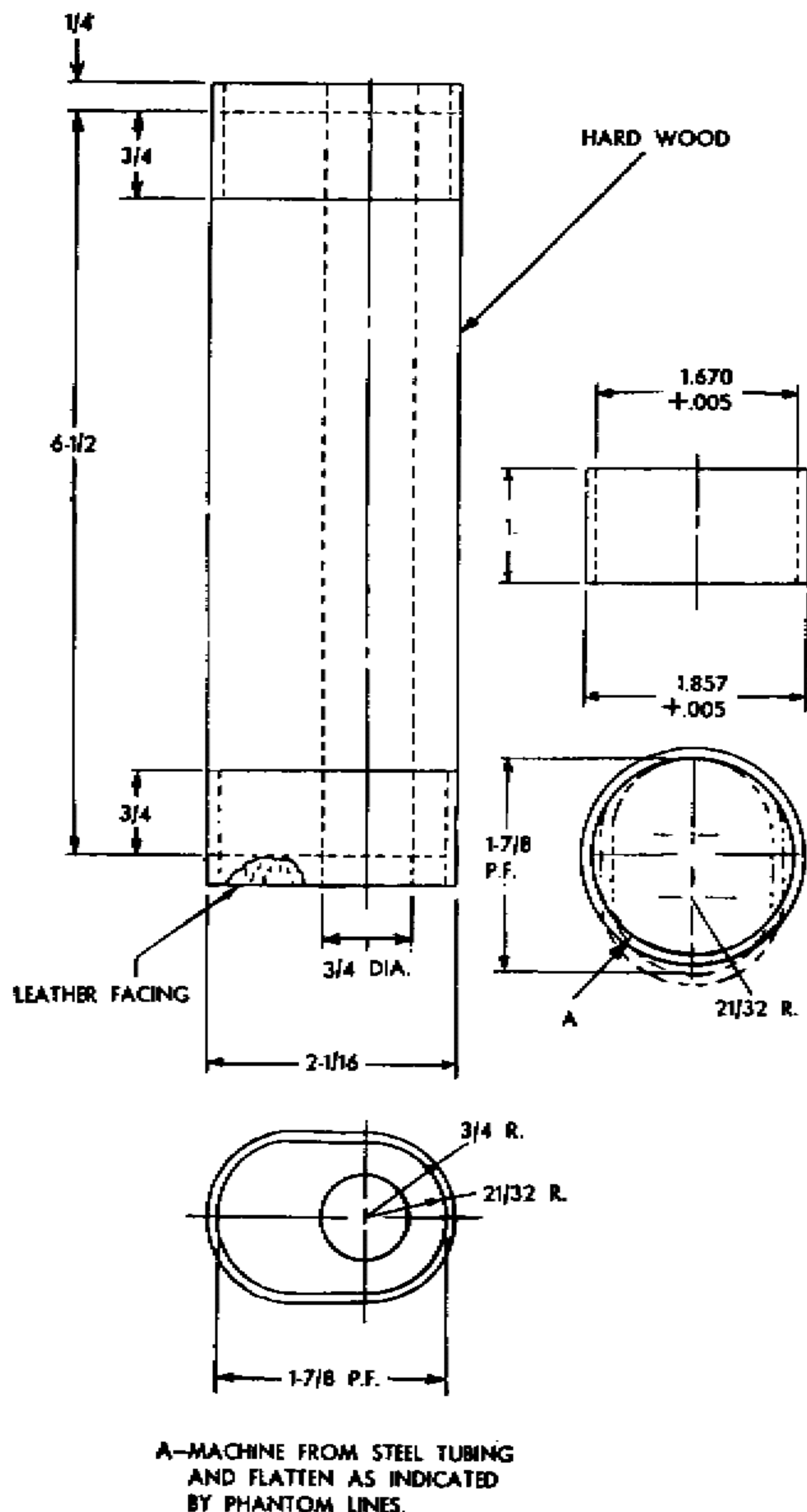
Fig. 104. Lower band driver.
