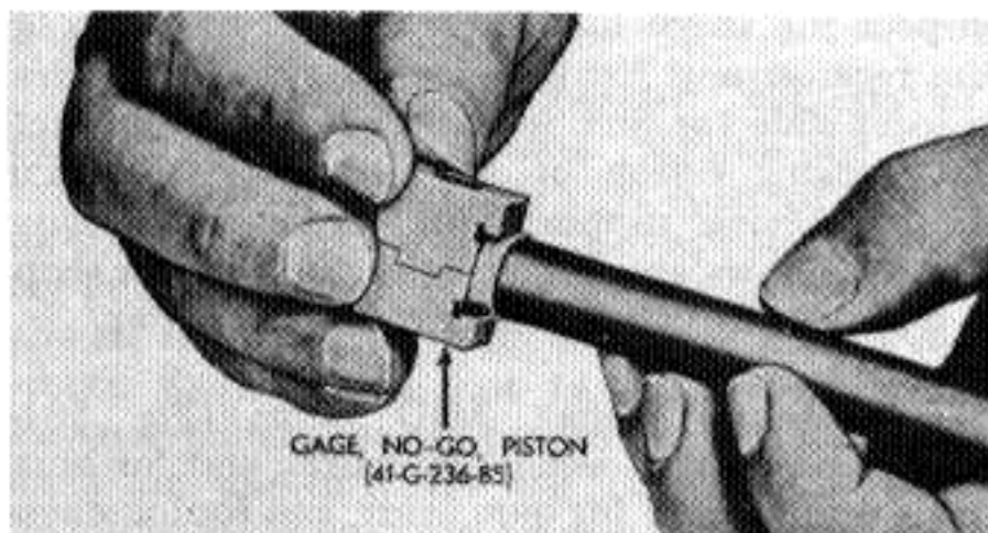
Fig. 122. Gaging diameter of piston.
