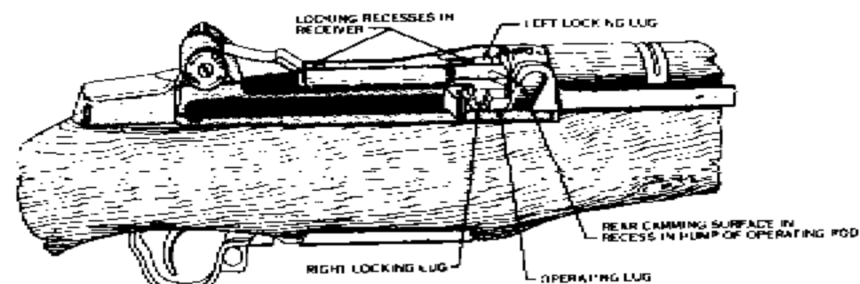
Fig. 50. Locking.
