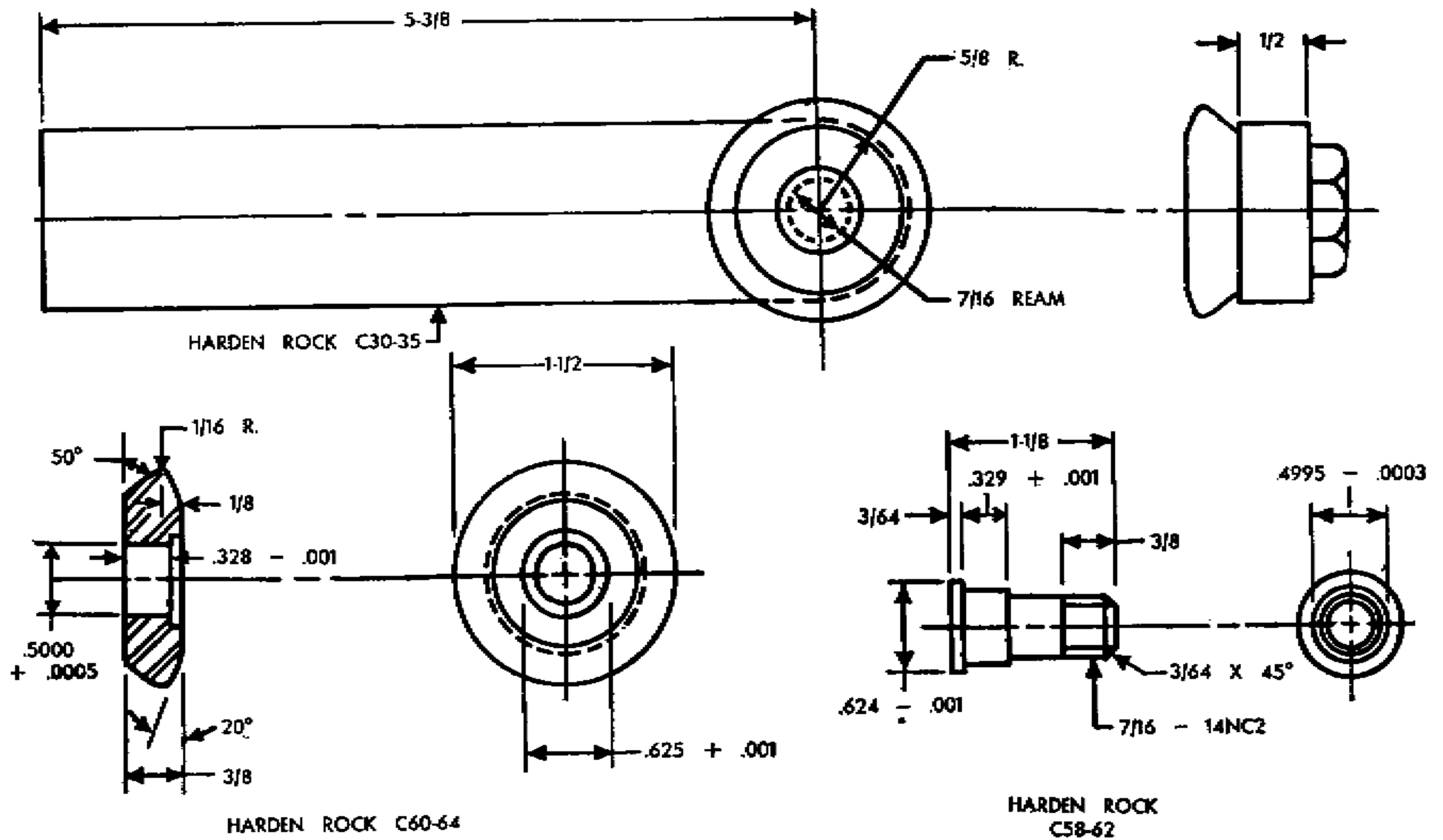
Fig. 108. Barrel & receiver swaging roll.
