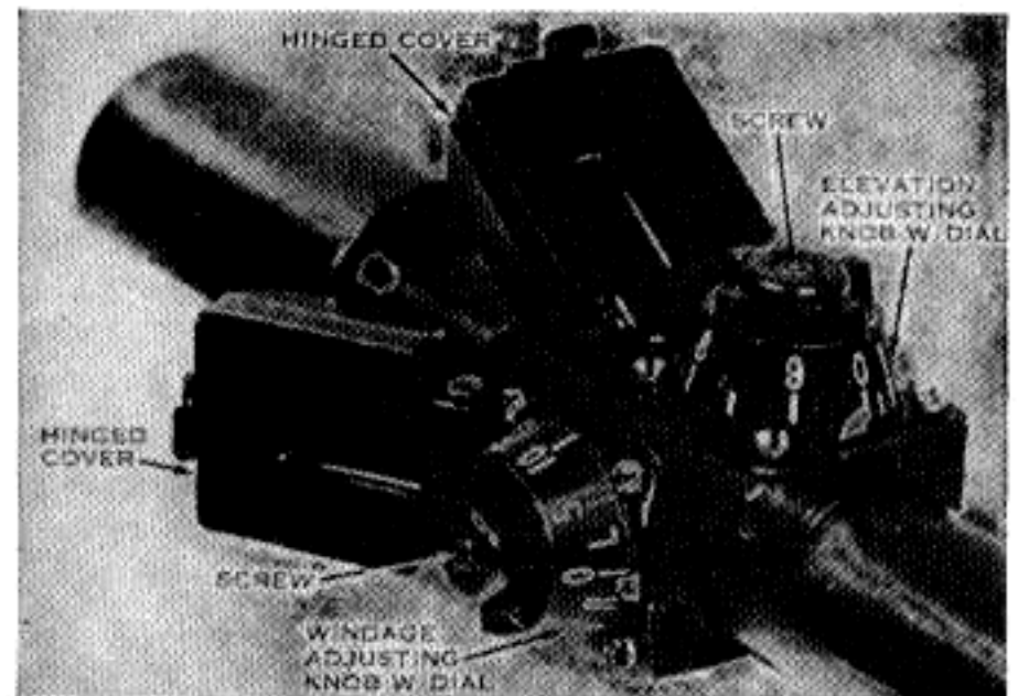
Fig. 13. Windage and elevation knobs, M84 scope.
