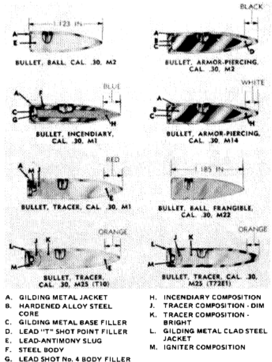
Fig. 26. .30 bullets cross-sectioned.
