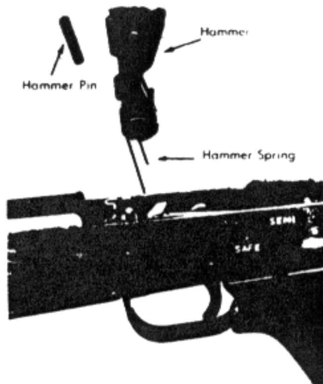
Remove/Install Hammer and Hammer Spring Figure 3-4
