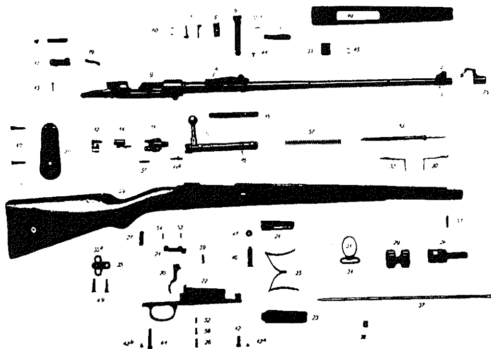
Component parts of the F. N. Rifle (Mauser System),
