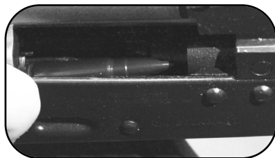
Round being stripped from magazine.
