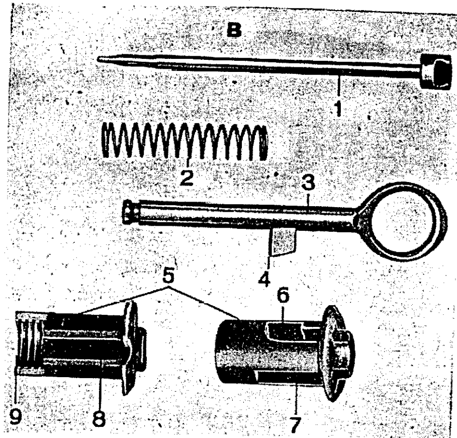
Fig. 12 Firing Mechanism
