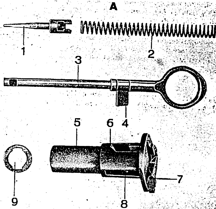
Fig. 11 Firing Mechanism
