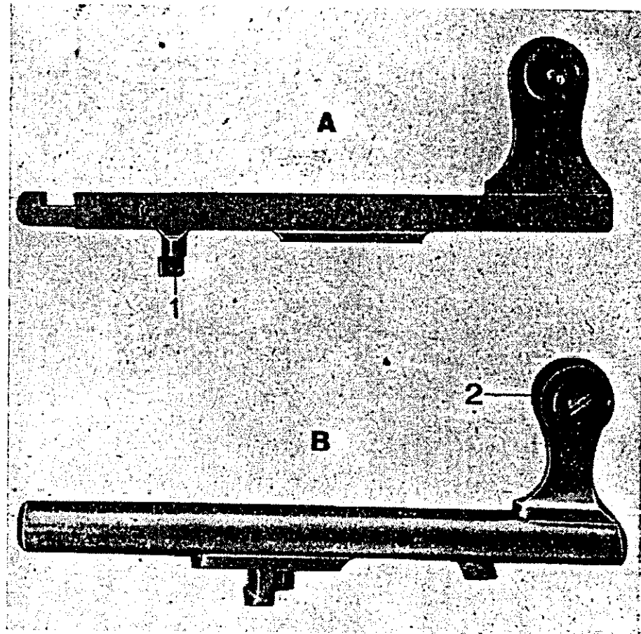
Figure 8 Cam Follower
