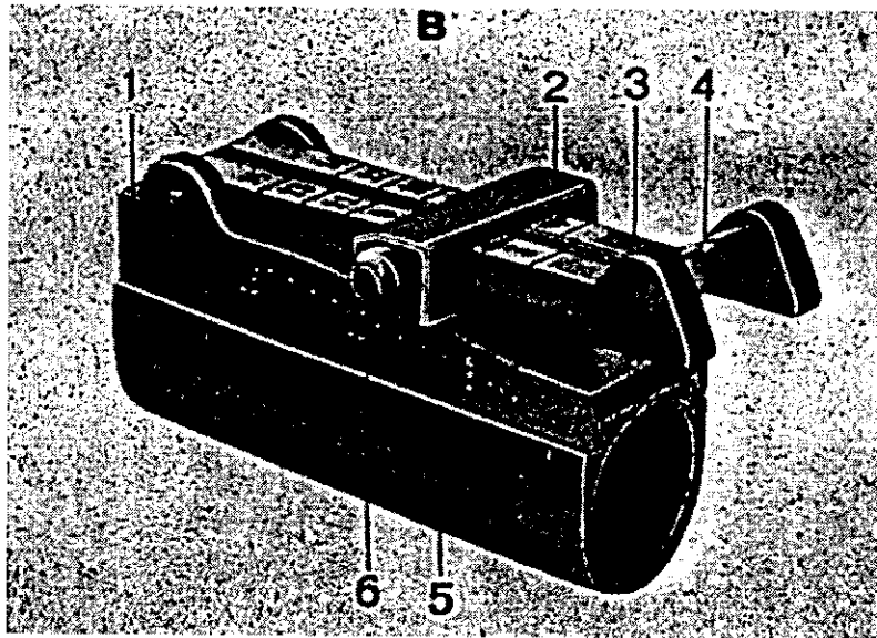
Figure 5 Rear Sight
