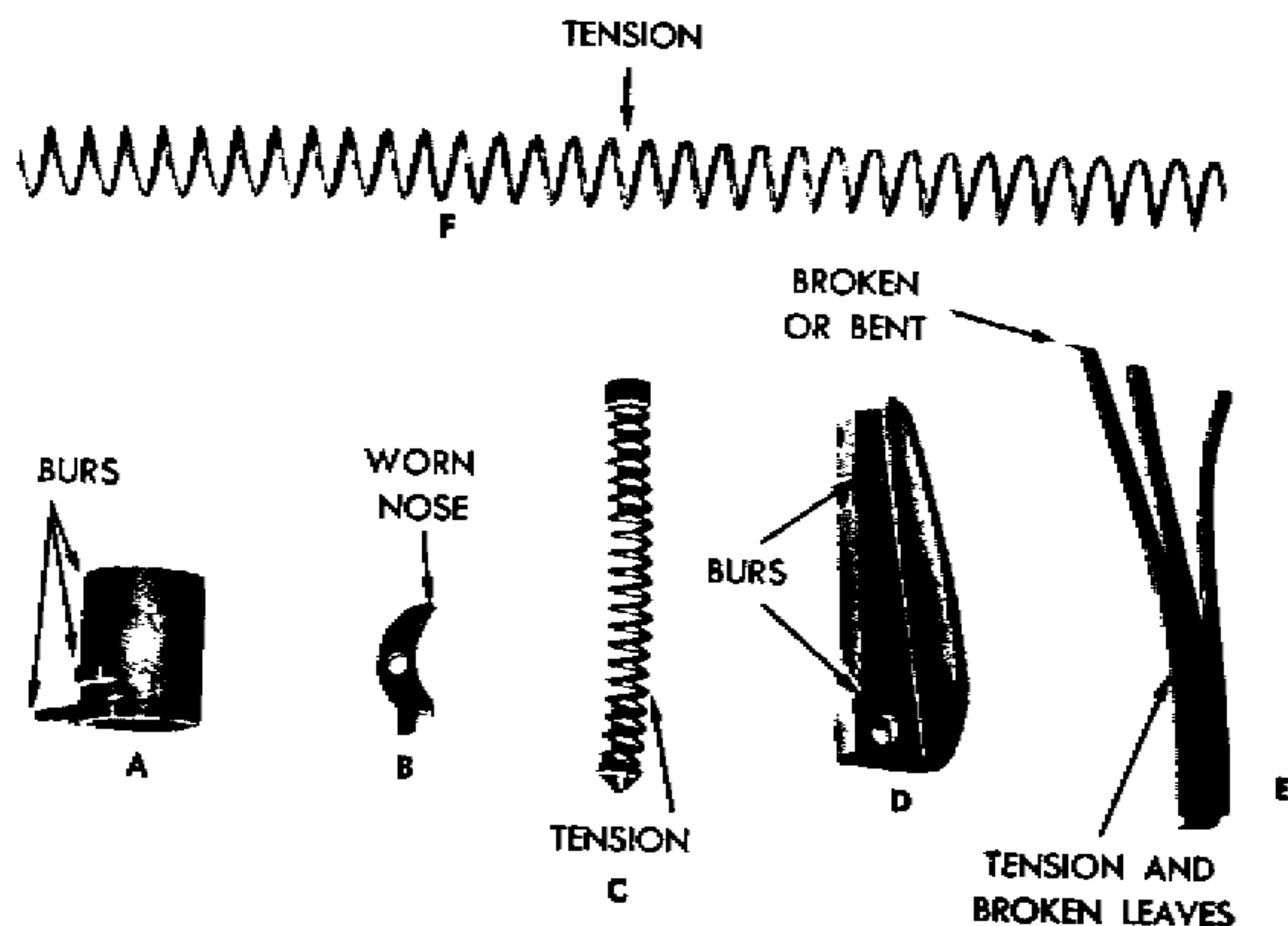
Figure 56. — Showing Points to Be Inspected On: a. Barrel bushing; b. Sear; c. Mainspring; d. Mainspring housing; e. Sear spring; f. Recoil spring
