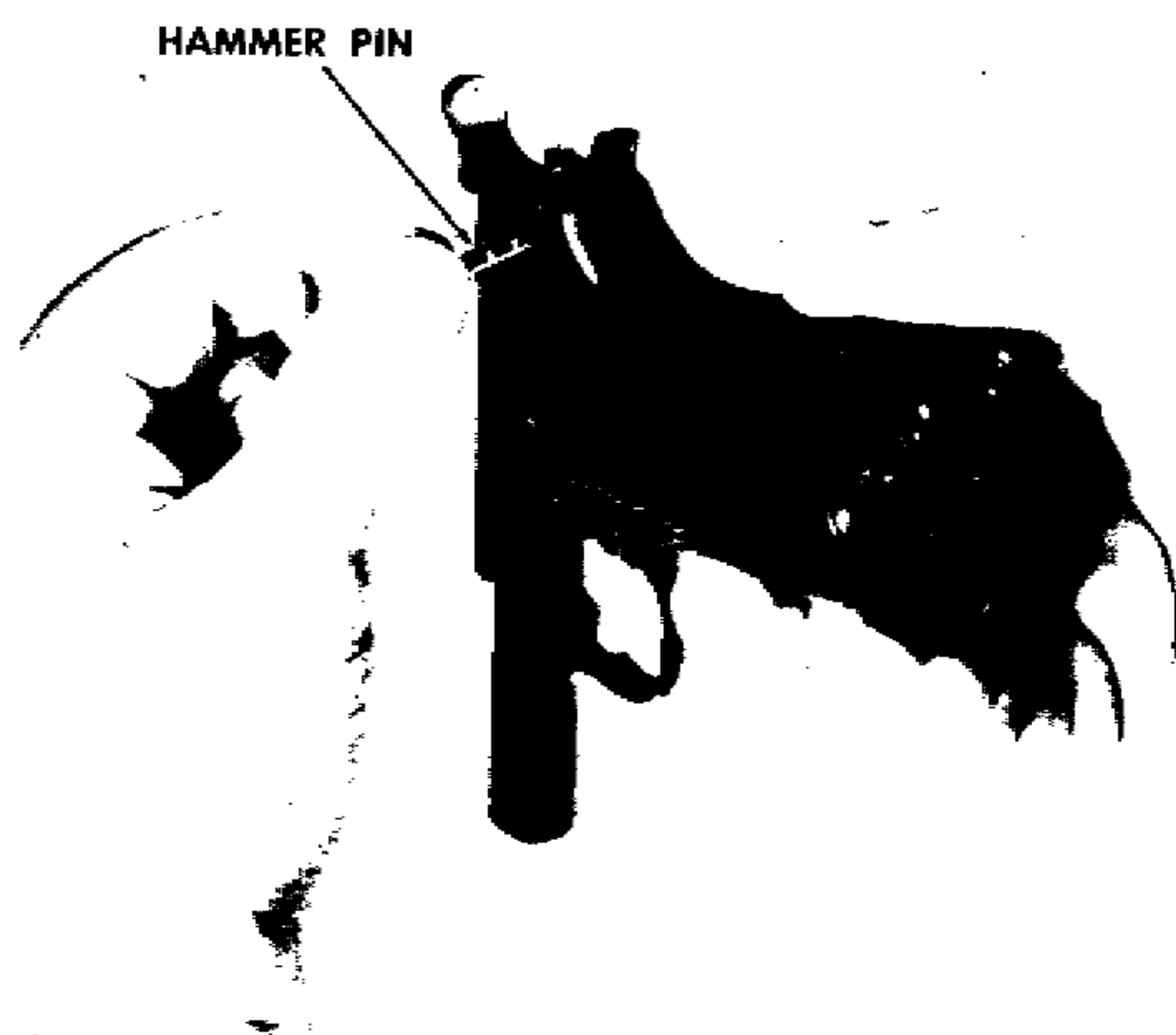
Figure 46. Remove the hammer pin from the left side of the receiver.
