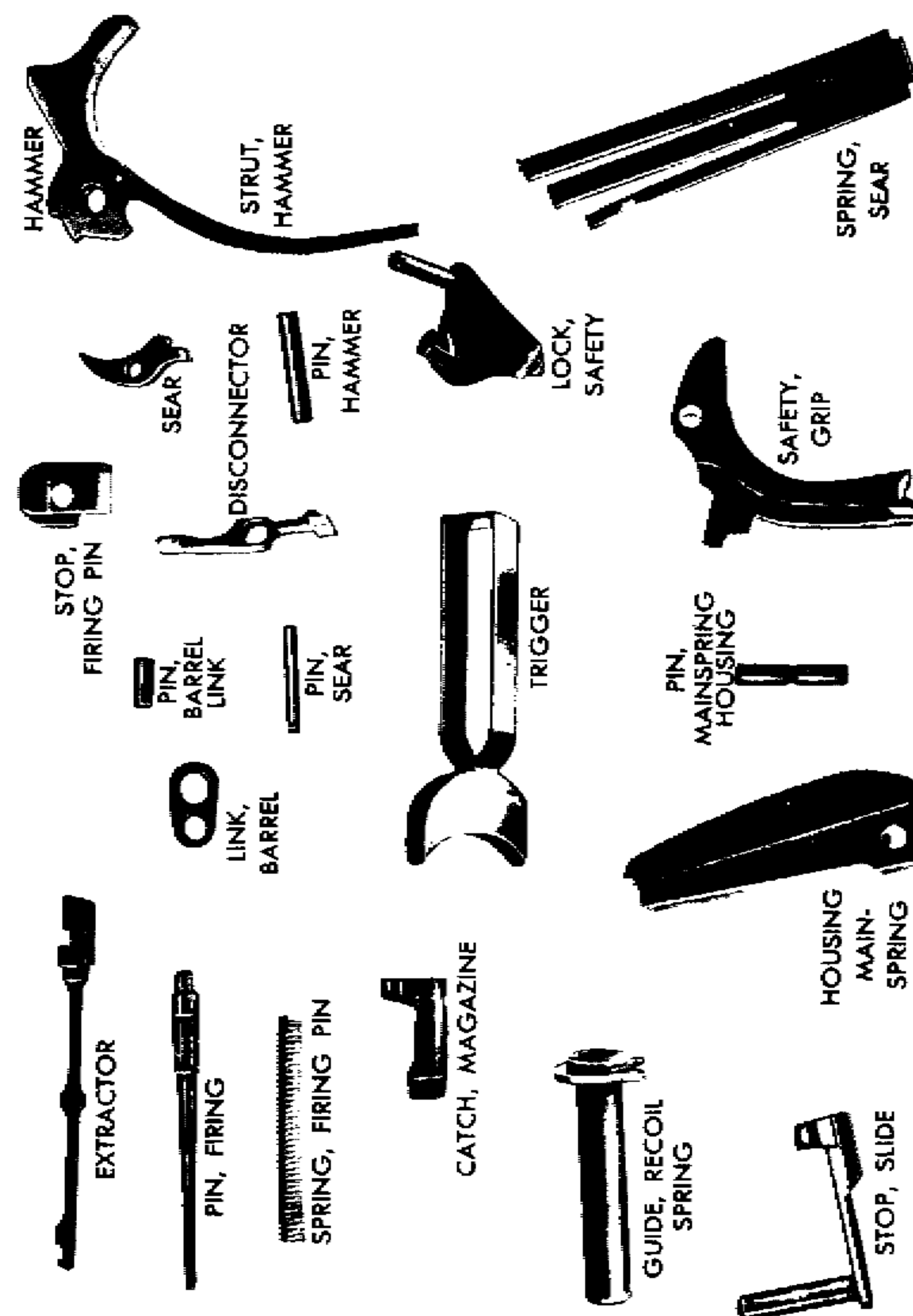
Figure 36. — Group of Smaller Parts of Pistol M1911A1
