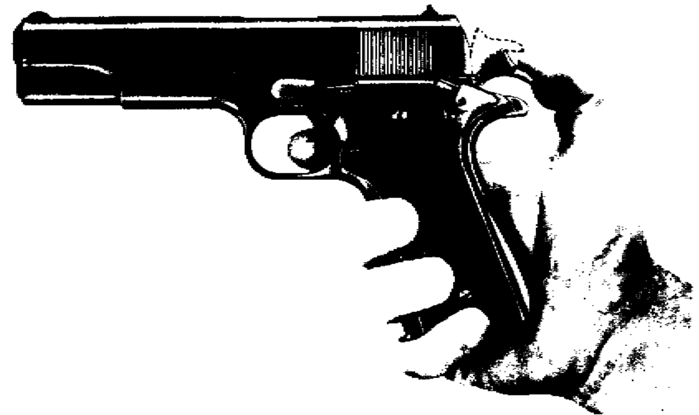
Figure 29. — Pistol M1911A1, Hammer at Half-Cock Notch, Finger Squeezing Trigger
