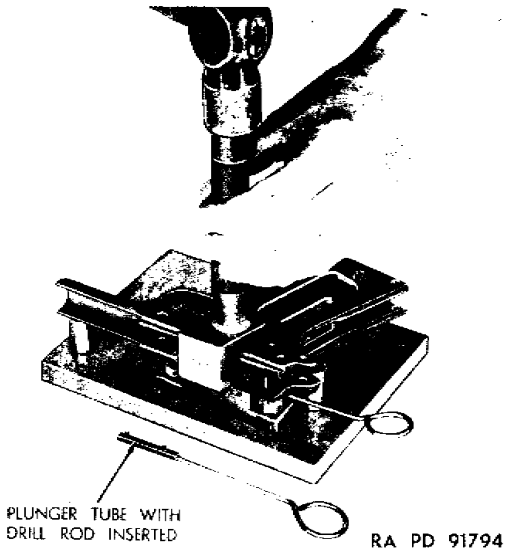
Figure 161. Staking slide stop plunger tube.
