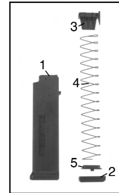
Fig. 13 Magazine, disassembled
