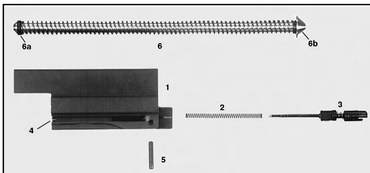
Fig. 9 Bolt Group, disassembled
