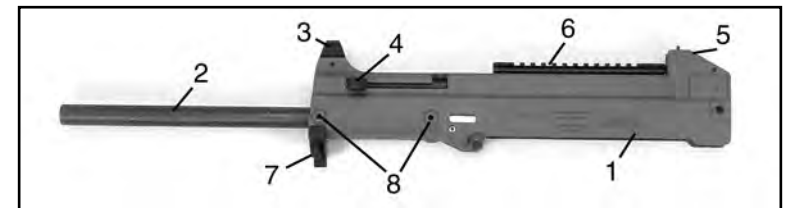
Fig. 5 Upper Receiver with barrel and attachment components
