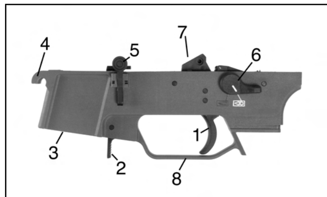
Fig. 10 Lower receiver with trigger mechanism and magazine well
