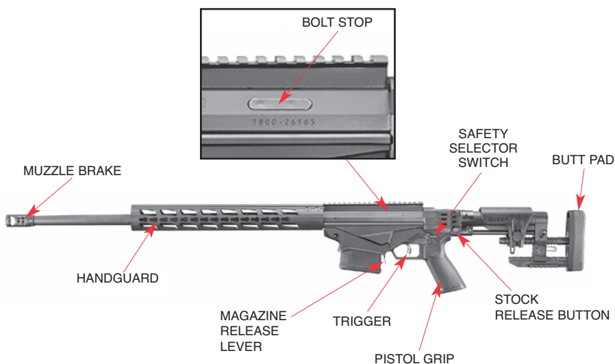
Figure 3 – In these illustrations the frequently used operating components are identified.
