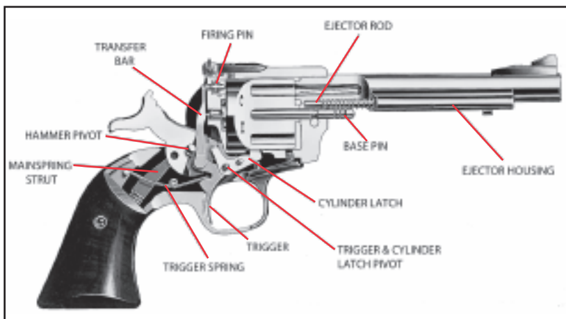
Figure 4. Mechanism shown with trigger pulled and hammer beginning to fall. Transfer bar is in firing position, between hammer and firing pin.
