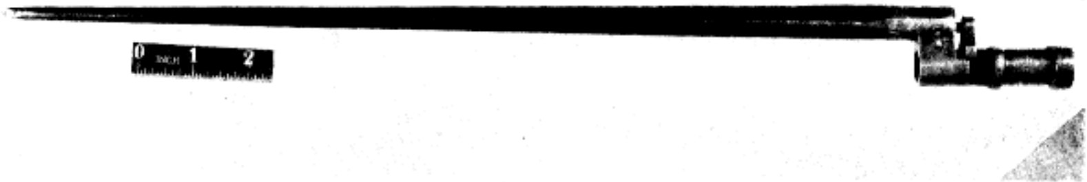
FIGURE 19. BAYONET FOR RIFLE M1891/30.
