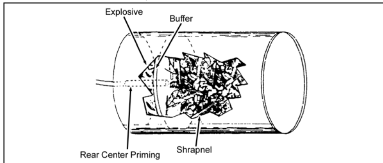
Figure 13-4. GRAPESHOT CHARGE
