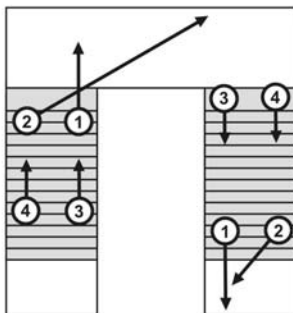
Figure 6-17. CLOSED STAIRWELL
