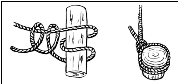
Figure 10-6. ROUND-TURN WITH TWO HALF-HITCHES
