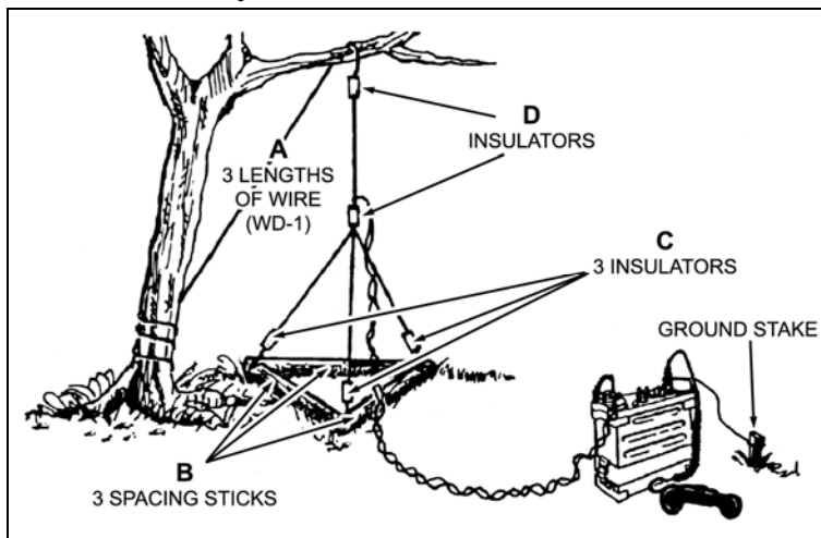
Figure 7-9. COMPLETE EXPEDIENT 292-TYPE ANTENNA
