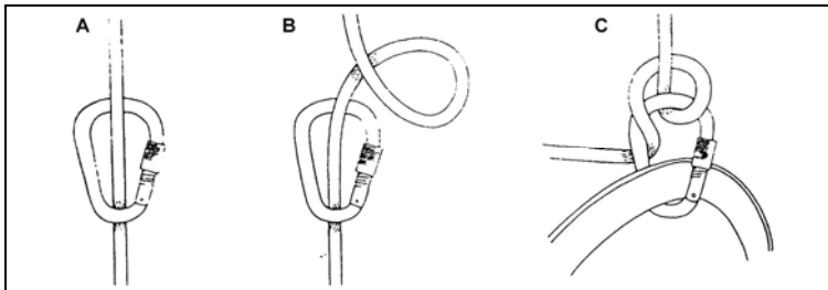
Figure 10-18. MUNTER HITCH
