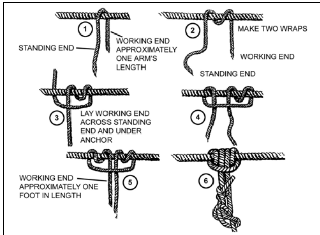
Figure 10-13. END-OF-THE-ROPE PRUSIK
