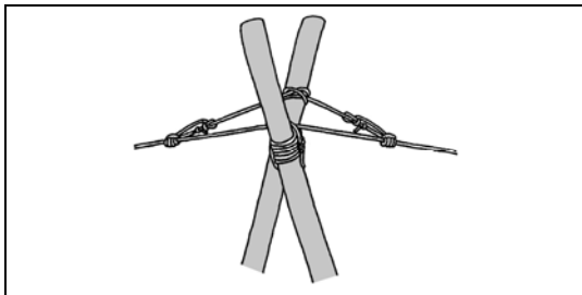
Figure 10-25. ANCHORING THE TRAVERSE ROPE TO THE A-FRAME
