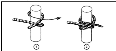
Figure 10-7. END-OF-THE-ROPE CLOVE HITCH
