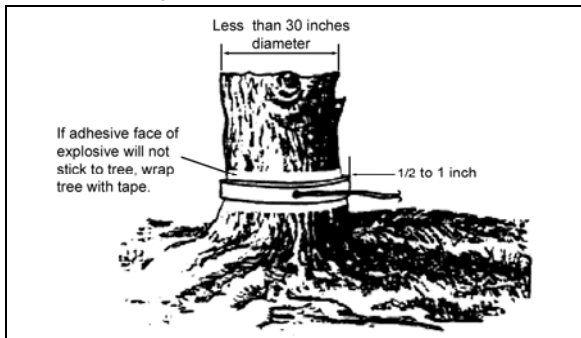
Figure 13-11. TIMBER-CUTTING RING CHARGE
