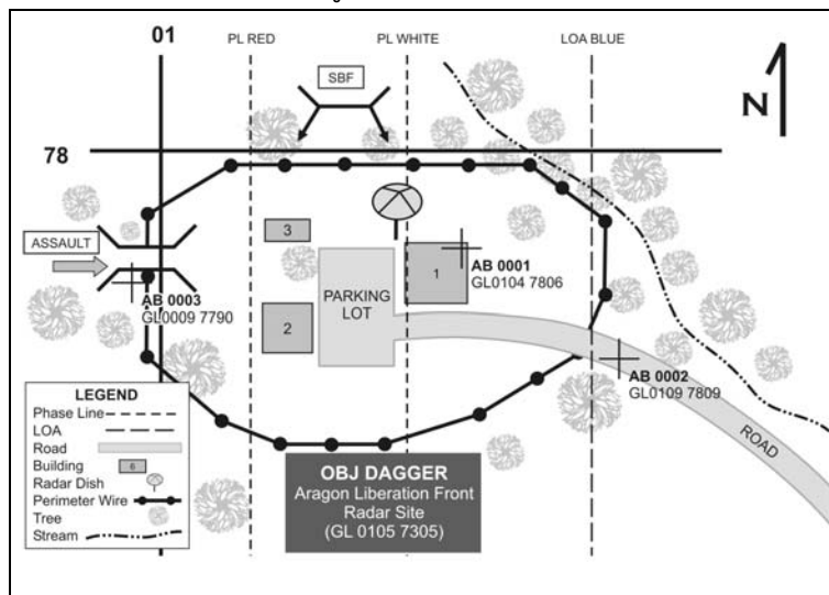
Figure 2-15. TERRAIN MODEL
