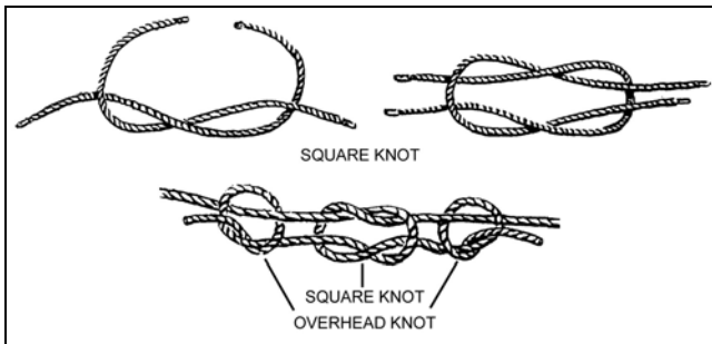
Figure 10-5. SQUARE KNOT
