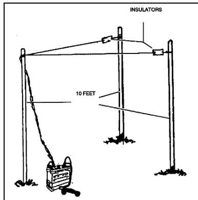
Figure 7-12. VEE ANTENNA
