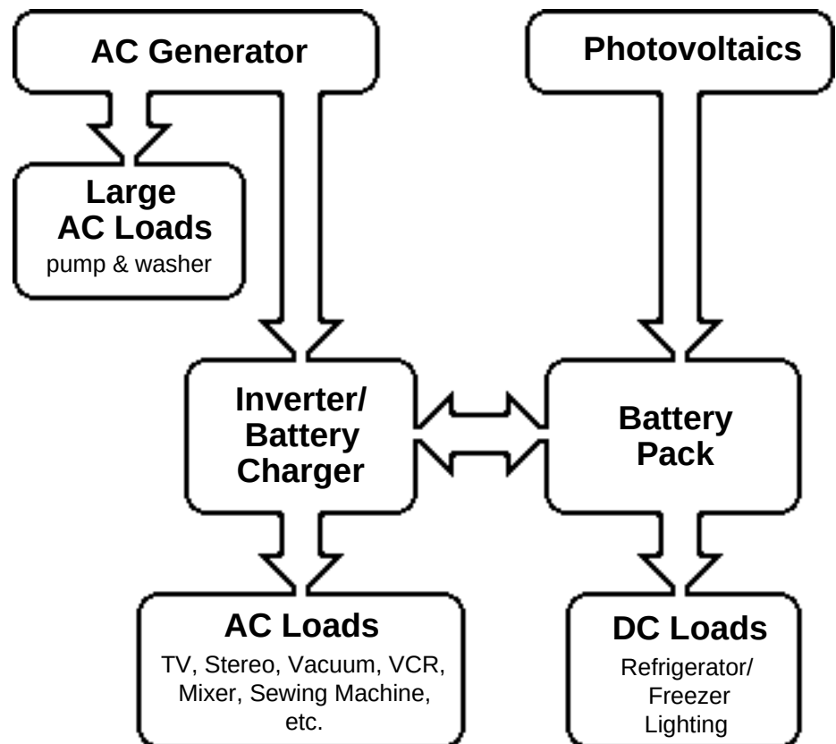
Figure 2 Smiths' Alternative Energy System
