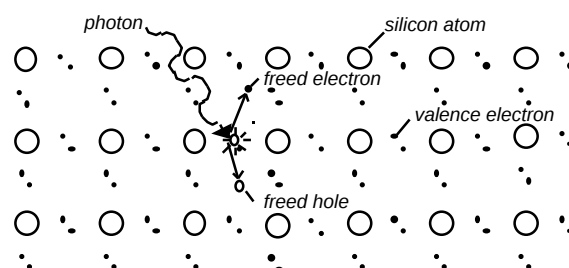
Figure 1 Photoconductive effect in silicon
