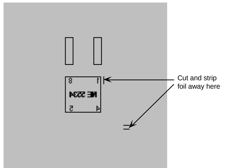
Foil Side
