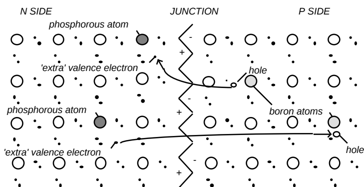
Figure 4 Junction forming
