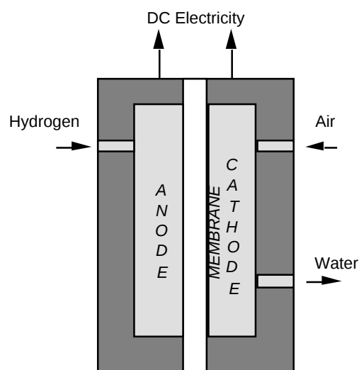
Diagram of PEM cell: The Proton Exchange Membrane Fuel Cell has platinum impregnated electrodes either side of a plastic film electrolyte.
