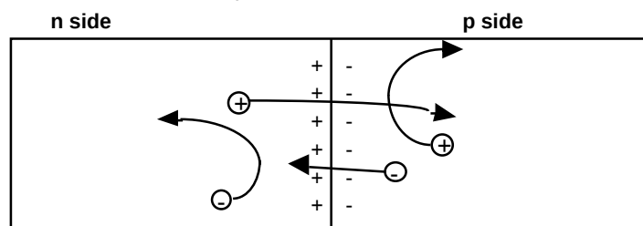
Figure 5 junction formed
