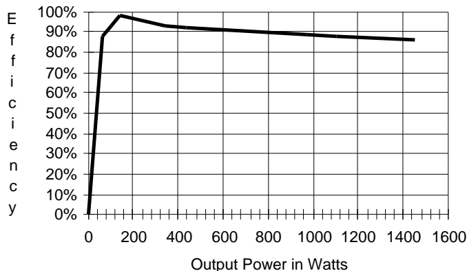
Efficiency vs. Output Power for Trace 2012 Inverter
