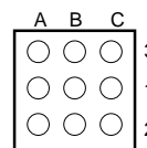
PIN CONNECTIONS FOR THE 3-POLE DOUBLE-THROW SWITCH (REAR VIEW)
