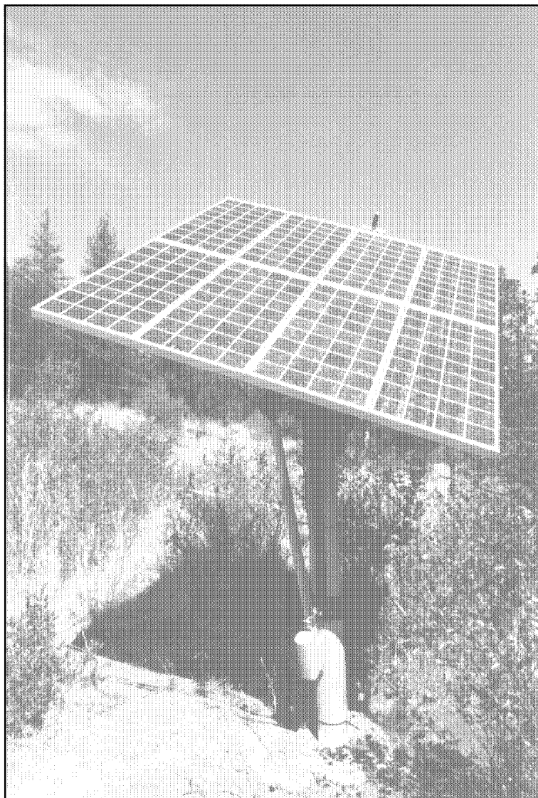
Above: A Wattsun two-axis PV tracker with eight Kyocera K51 modules aboard. The tracker is supported by a five inch steel pipe set four feet into the ground with cement.
