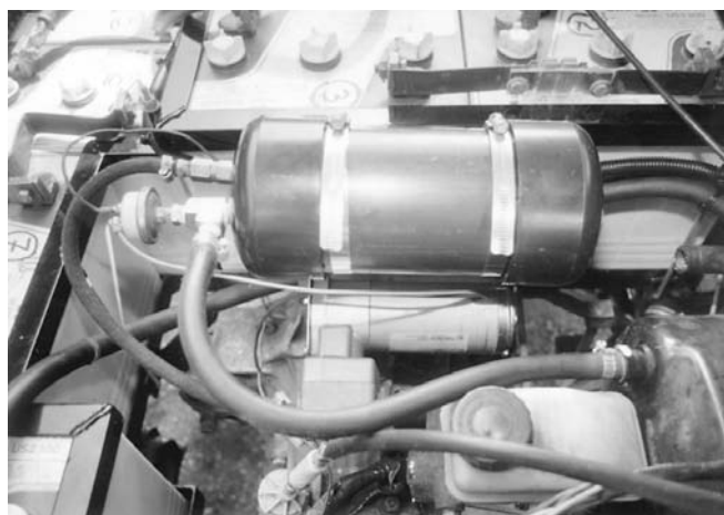
Above: A vacuum pump, reservoir, and switch provides power brakes in a VW Rabbit.
