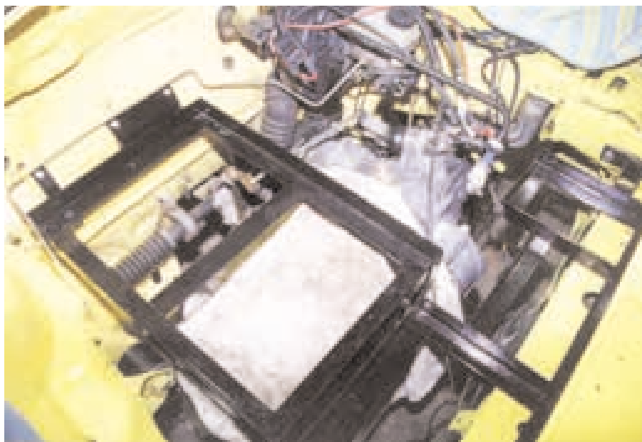
A split-level bridge rack supported on the right by the original bumper bracket bolts, and in the rear by the mount plate on the firewall.
