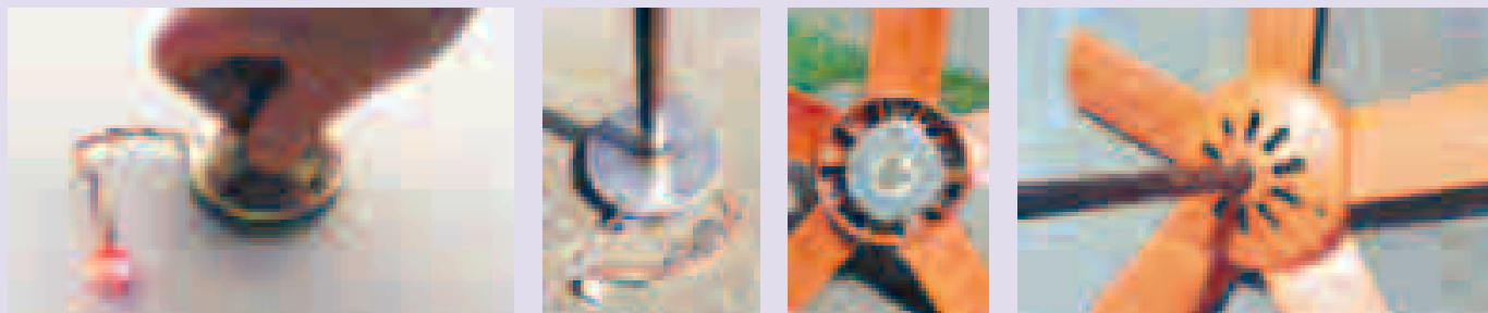
From left to right: Testing the stepper motor with LEDs. Fitting the windmill's shaft onto the motor. Installing the stepper motor inside the fan. Shaft attached to the fan, and facing the right direction.
