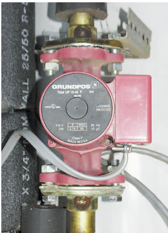
The Grundfos UP 15-42 F is a typical AC circulating pump for closed loop systems.
