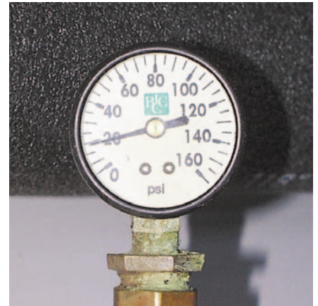
A pressure gauge can show leaks in the loop.
