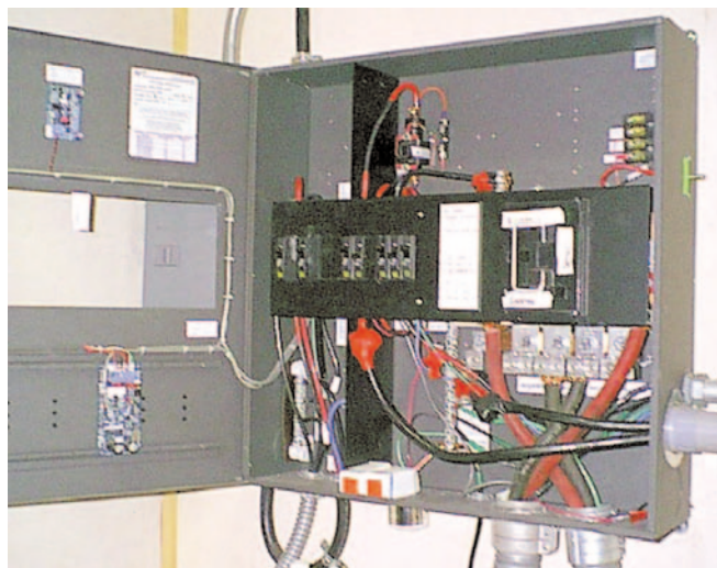
Inside the Ananda Power Center you can see the main pullout DC disconnect, DC breakers, and the backs of the TriMetric and Smart Charger.
