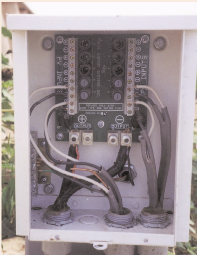
The Trace TCB10 PV combiner box provides fusing for each series string of photovoltaic modules.
