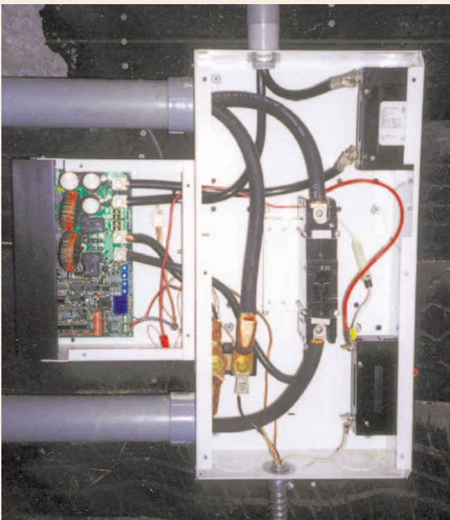
Inside the SB50 and DC250.
