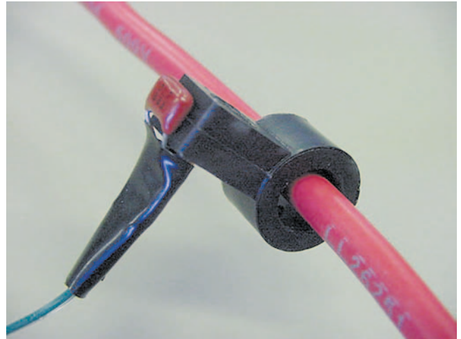
Close-up of the Hall-effect sensor and stabilizer capacitor. A major advantage of the Hall-effect current sensor is its isolation. It may be placed on either the positive or negative line. It is shown here measuring current in a positive line.
