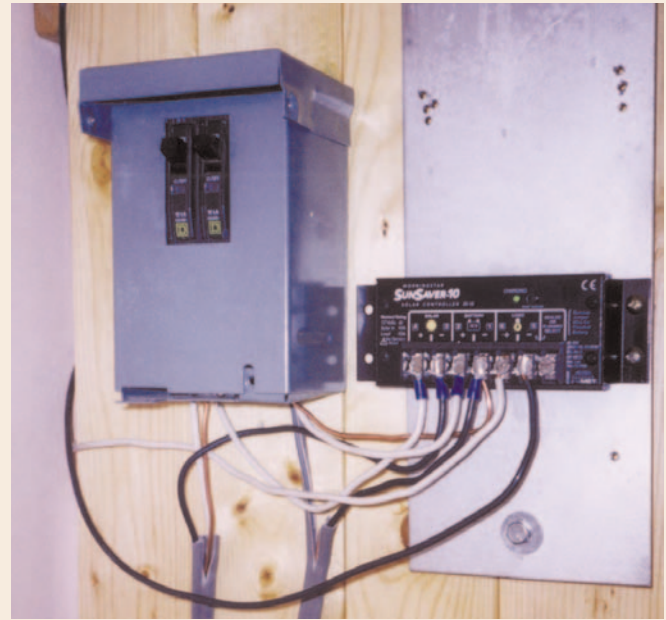
Breakers and the Morningstar SunSaver-10 charge controller for the 12 volt system.
