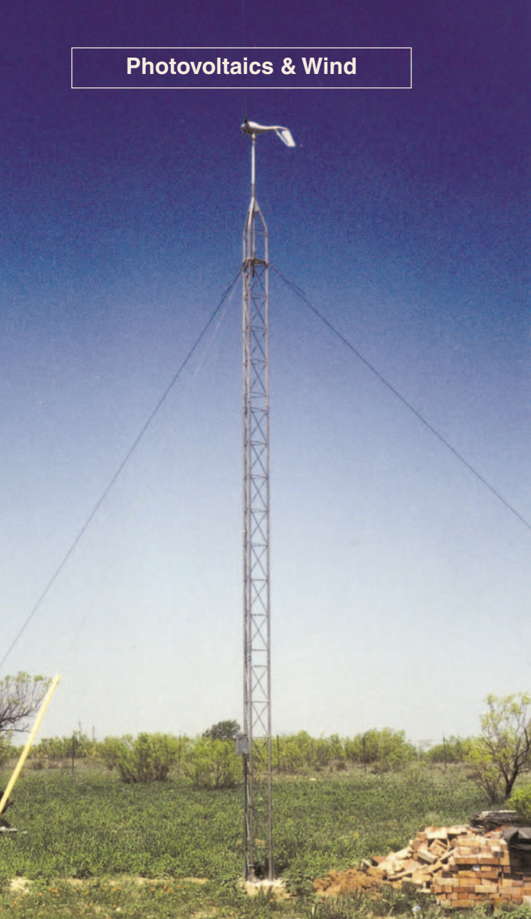
The Southwest Windpower Air 403 on a 30 foot tall Rohn 25G tower.
