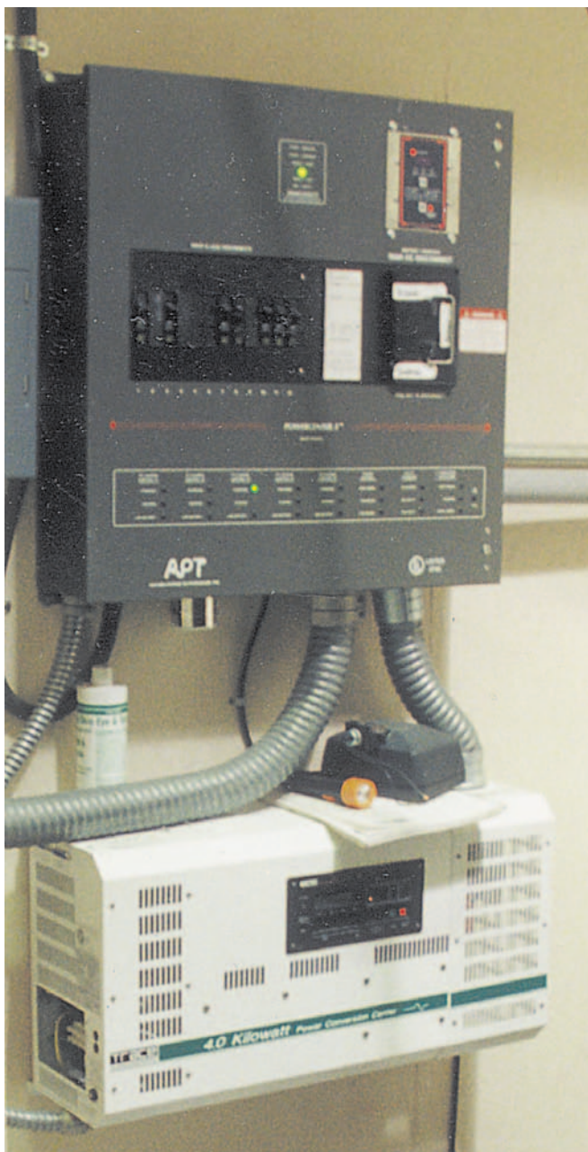
The Ananda Power Center and Trace SW4024 came prewired and were bought used.
