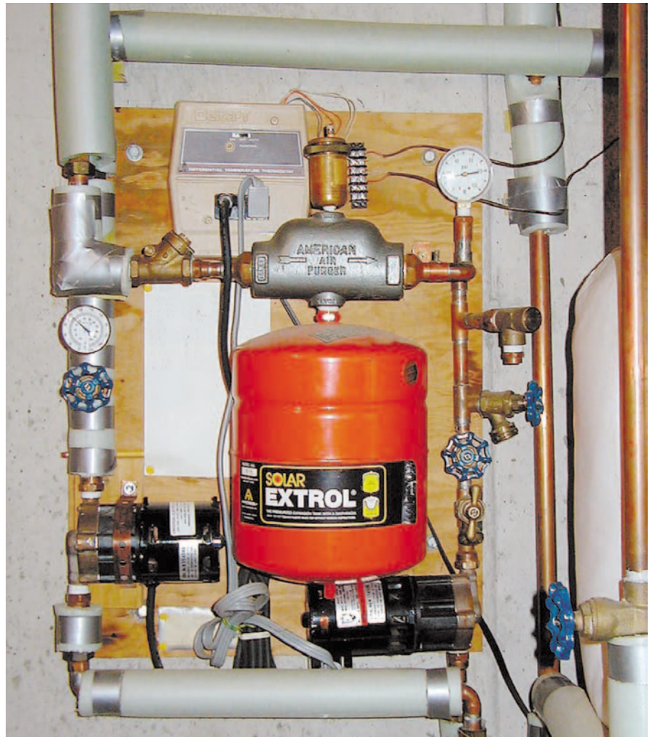
A closed loop module groups the major components on one board. This homebrew model by the author has functioned without fail since 1982.
