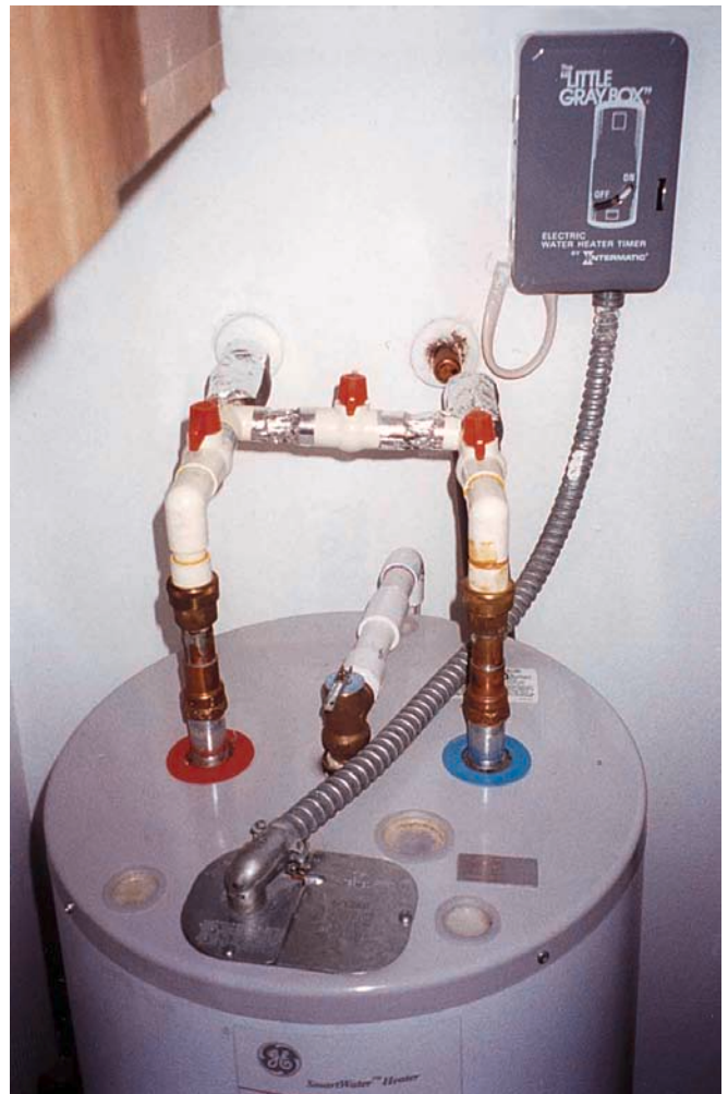
On the electric water heater, the timer switch and bypass valves are arranged for easy access.
