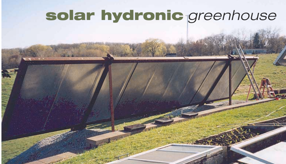
The 8 by 40 foot maxi-collector is all one unit, custom built for the greenhouse.
