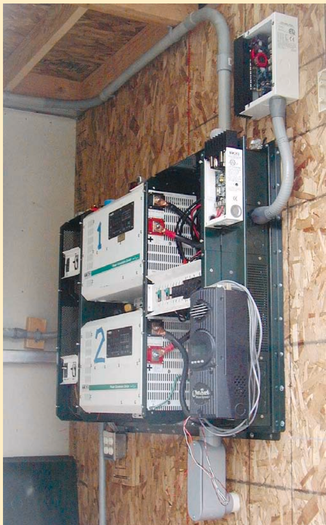
Colorado's power system—two Trace SW5548 inverters, Solar Boost 3048, Trace C40 and Outback MX-60 charge controllers, and Outback power system enclosure.
