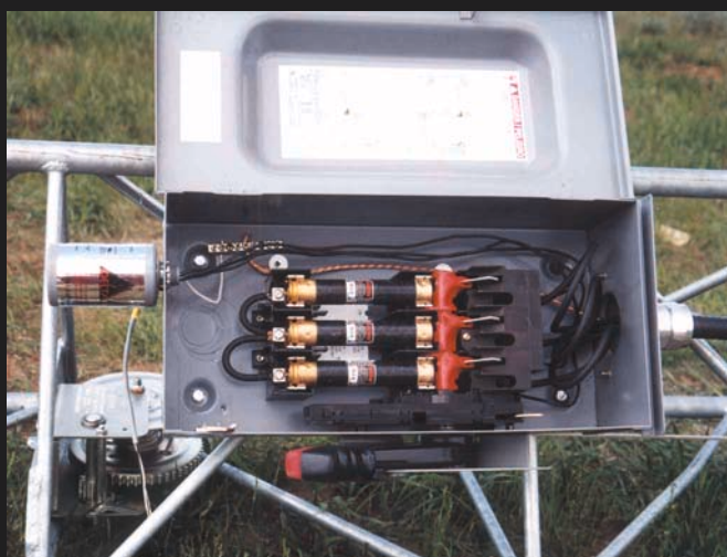
Overcurrent protection at the tower's base.
