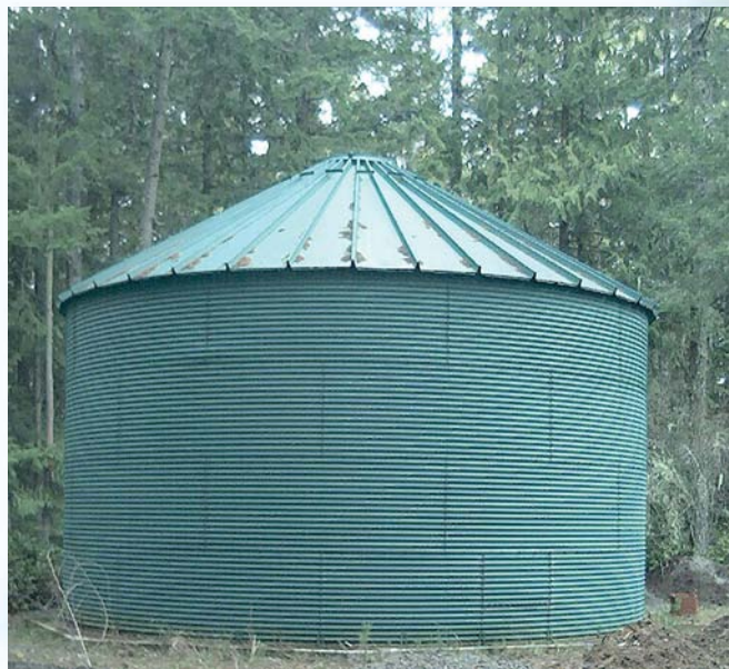
This 27-foot-diameter, 14-foot-tall, steel storage tank, lined with an FDA-approved PVC liner, can store about 58,000 gallons of rainwater.
