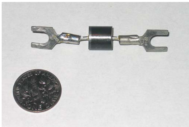
A small bypass diode from a 75-watt photovoltaic module.
