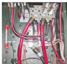
Use bus bars to parallel multiple series strings.
