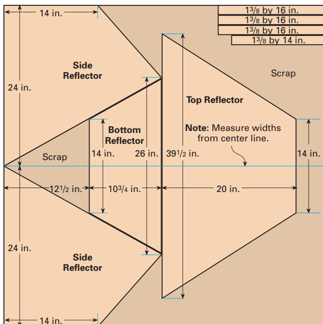
Hardboard: 4 by 4 ft., \frac{1}{8} in. thick
