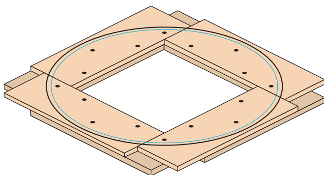
Two Layers Glued & Nailed Together
