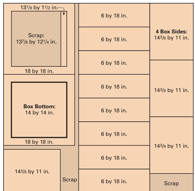
Plywood: 4 by 4 ft., \frac{3}{8} in. thick
