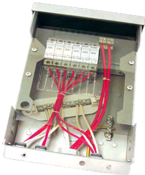
Combiner boxes, like this one from OutBack Power Systems, provide necessary overcurrent protection for the array.
