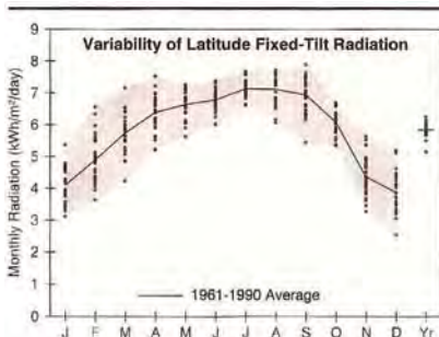
Solar Radiation for Flat-Plate Collectors Facing South at a Fixed Tilt (kWh/m 2 /day), Uncertainty \pm 9\%
