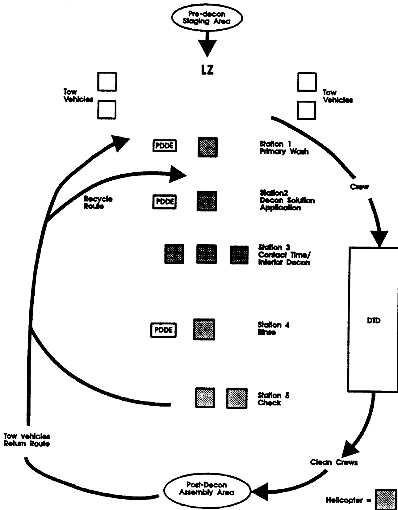
Figure 7-2. Optimum layout configuration of a detailed aircraft decon station.
