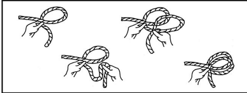
Figure G-5. Clove Hitch
