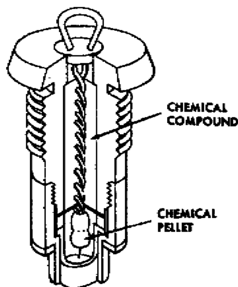
PULL-FRICTION FUZE, WEST WW II GERMANY
