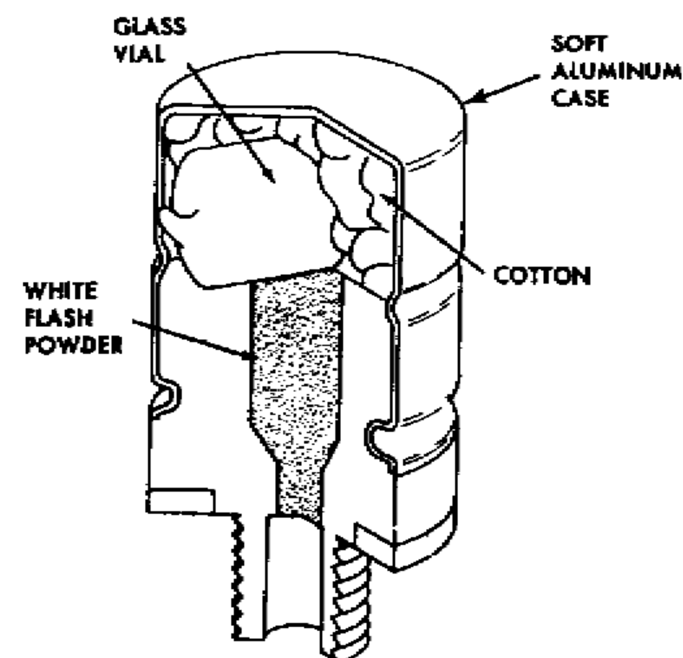
WW II GERMANY BUCK CHEMICAL FUZE
