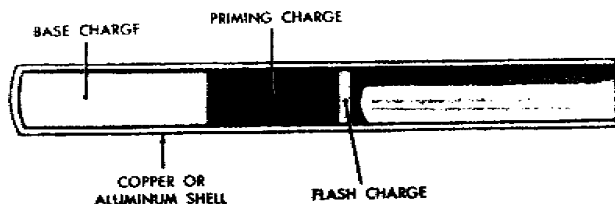
NON-ELECTRIC BLASTING CAP
