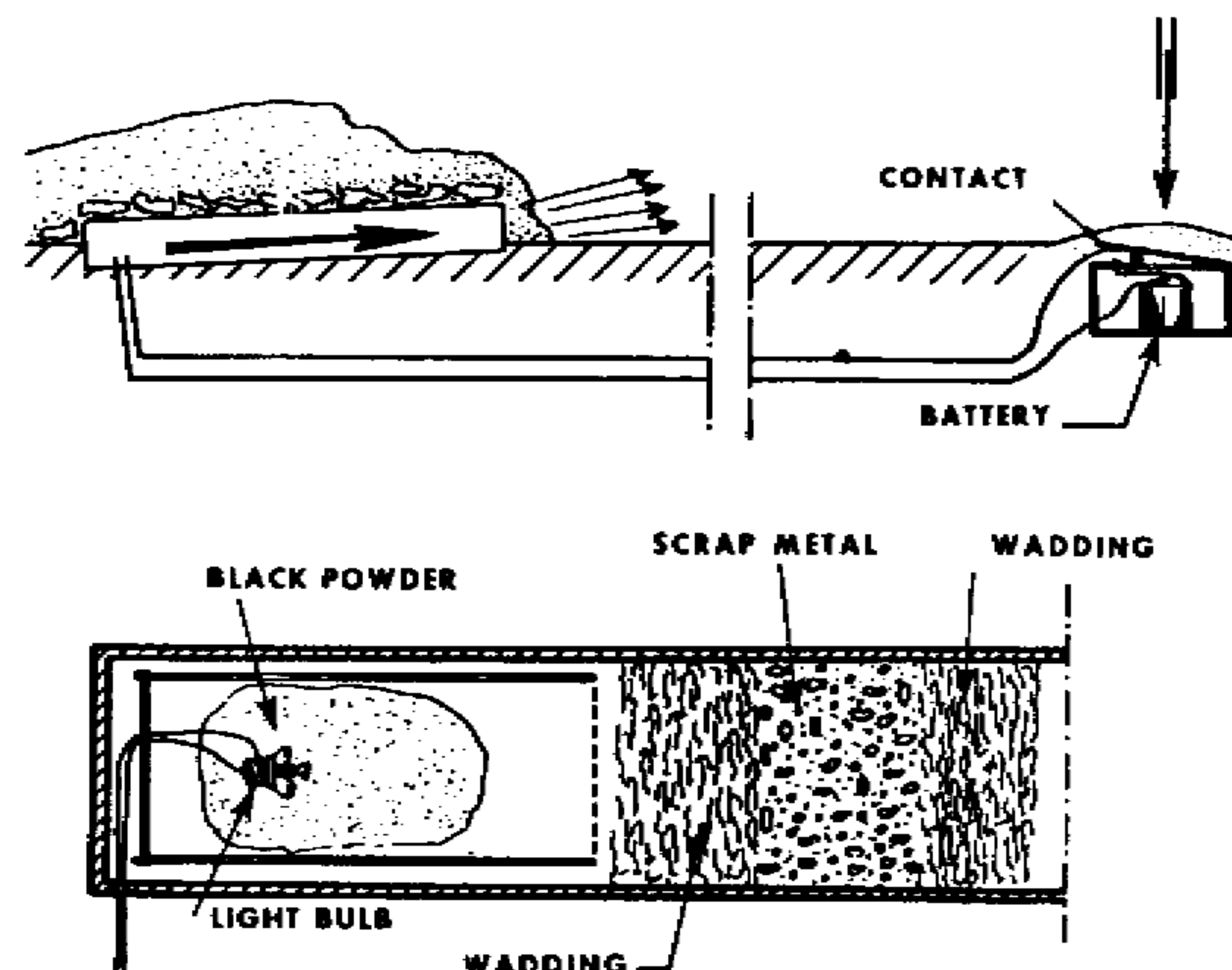
DETAIL OF EMPLACED EXPLOSIVE CHARGE
