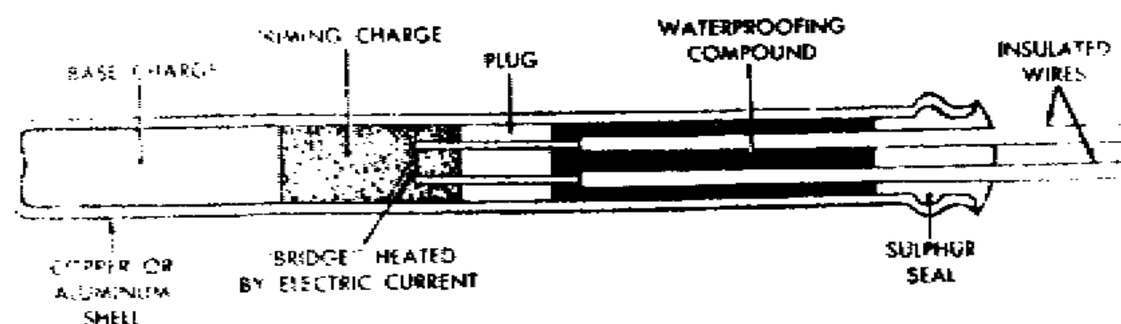
ELECTRIC BLASTING CAP
