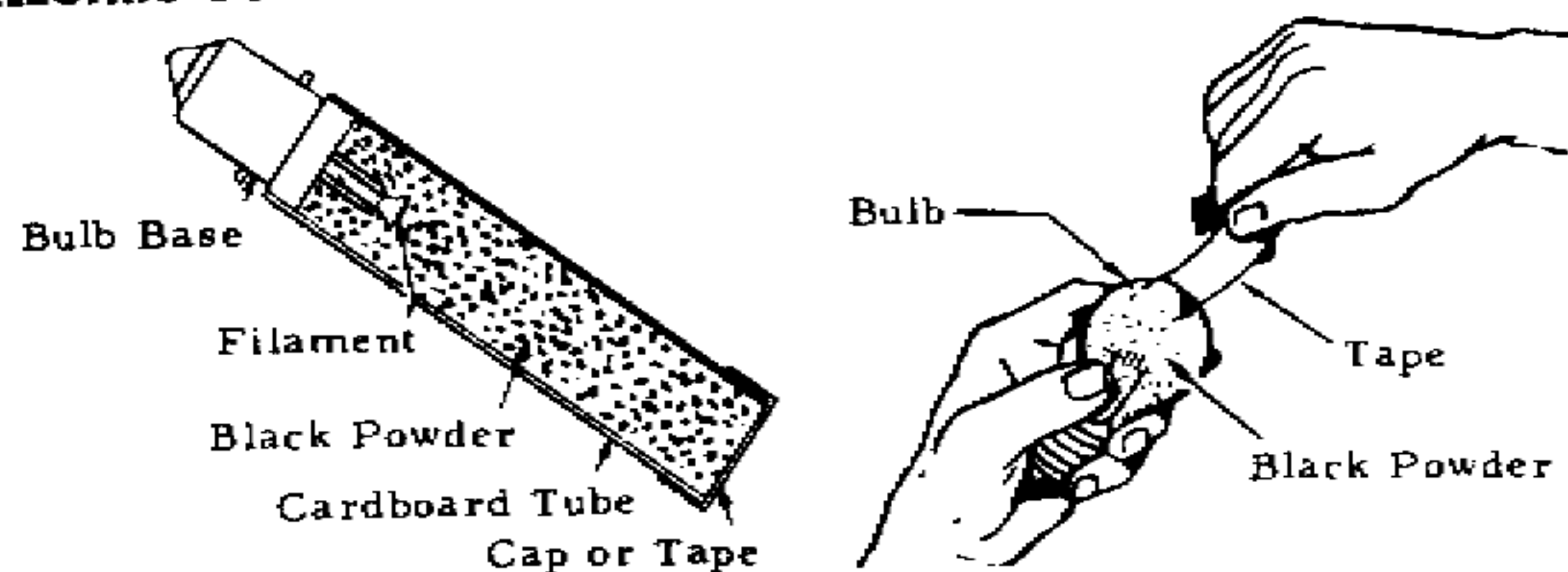
FILLED BULB DEVICE
