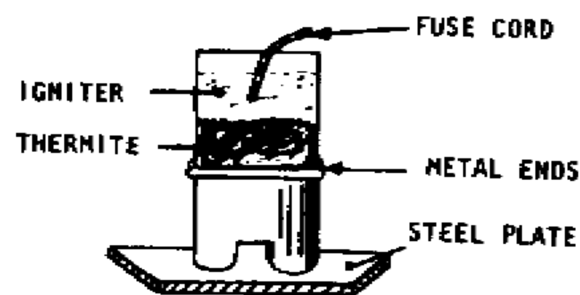
HOLE BURNING METHOD
